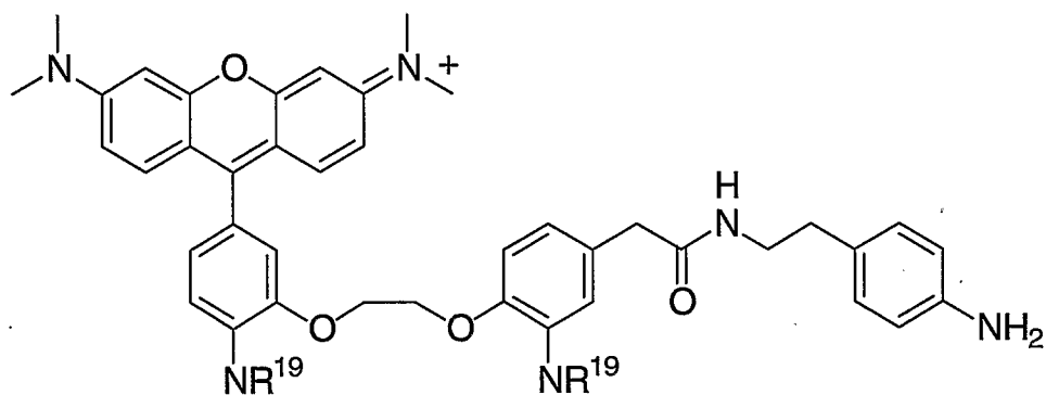
Compound 10,
