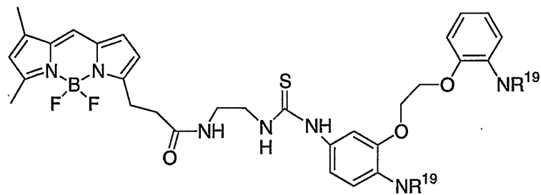
Compound 24,
