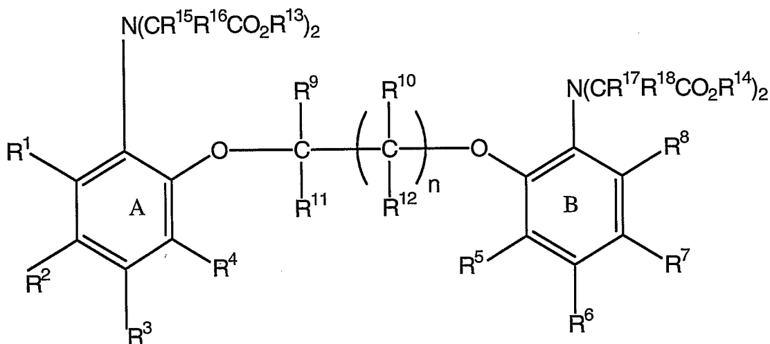
FORMULA IV
