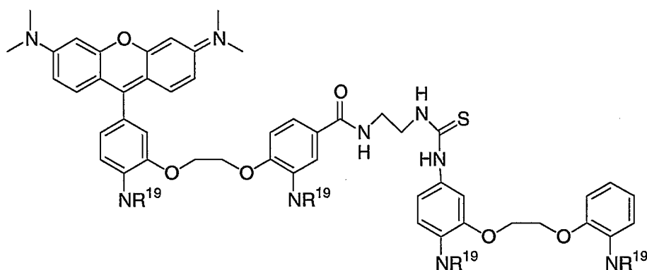
Compound 26 and
