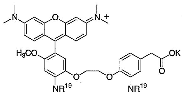
Compound 18,
