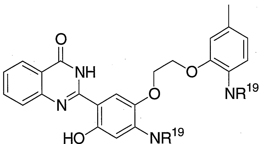
Compound 6,
