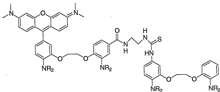
Compound 26
