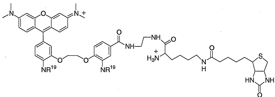
Compound 18,
