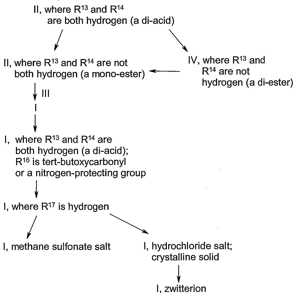
Scheme 2: Process for Preparation of Particular Salt
