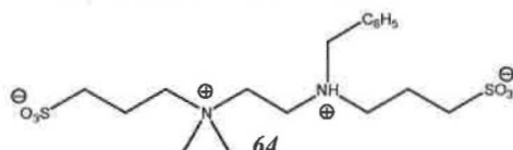
64 N,N-Dimethyl-N'-benzyl-N,N'-bis- (3-sulfopropyl)ethylenediammonium Di-inner Salt
