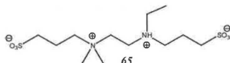
65 N,N'-Dimethyl-N'-ethyl-N,N'-bis- (3-sulfopropyl)ethylenediammonium Di-inner Salt
