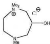
37 TIMOHOP 1,1,4-Trimethyl-6-hydroxy- homopiperazinium Chloride
