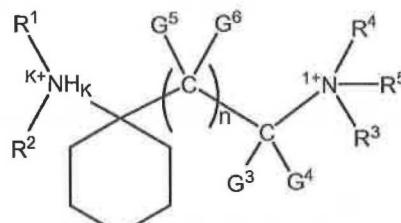
G^1G^2 pair; w=5 ; all ring G^1 and G^6 = H
