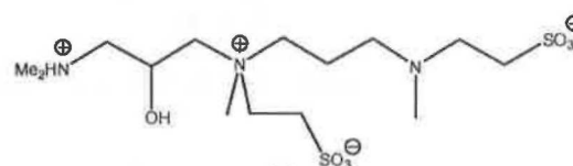
82 1,1,5,9-Tetramethyl-3-hydroxy-5,9-bis-(2-sulfoethyl)-1,5,9-triazanonane Di-inner Salt
