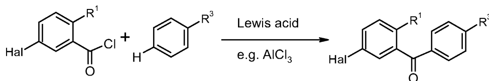
Scheme 2: Synthesis of the Diarylketone Fragment
