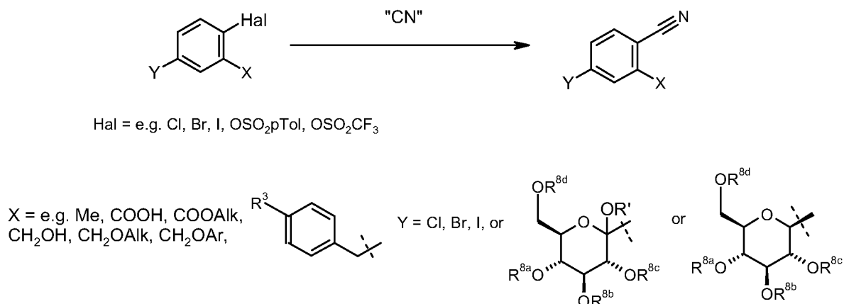
Scheme 5: Introduction of the Cyano Moiety
