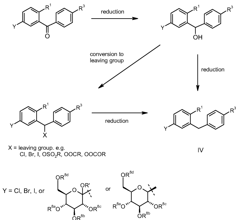
Scheme 3: Reduction of Diarylketones and Diarylmethanols to Diarylmethanes
