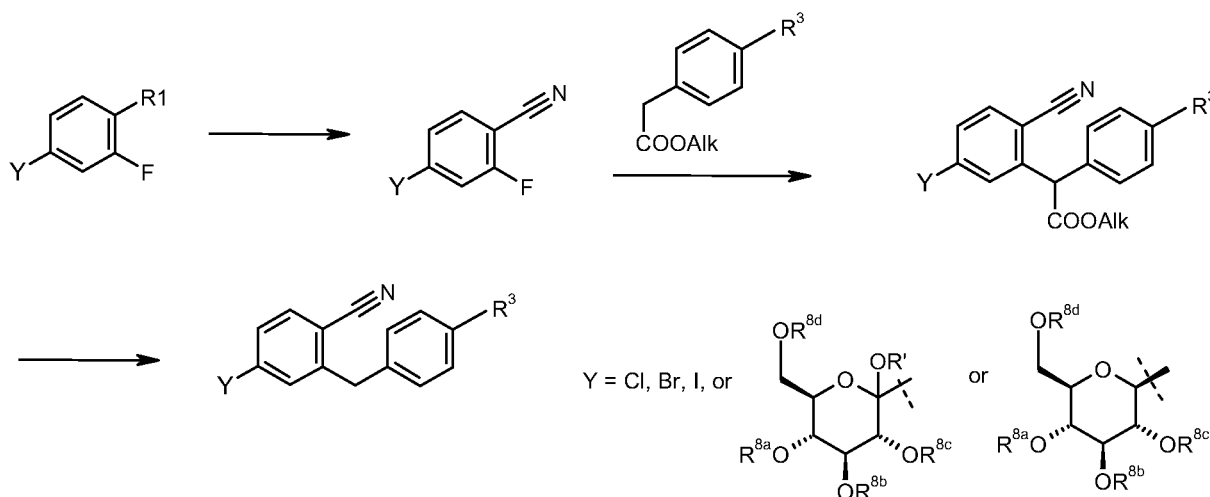
Scheme 8: Alternative Synthesis of Diarylmethane Unit
