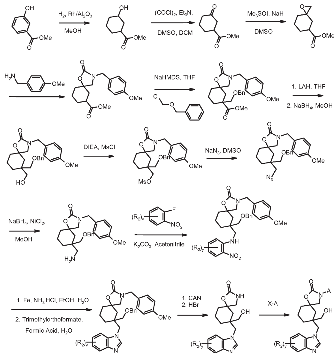
Scheme 8
