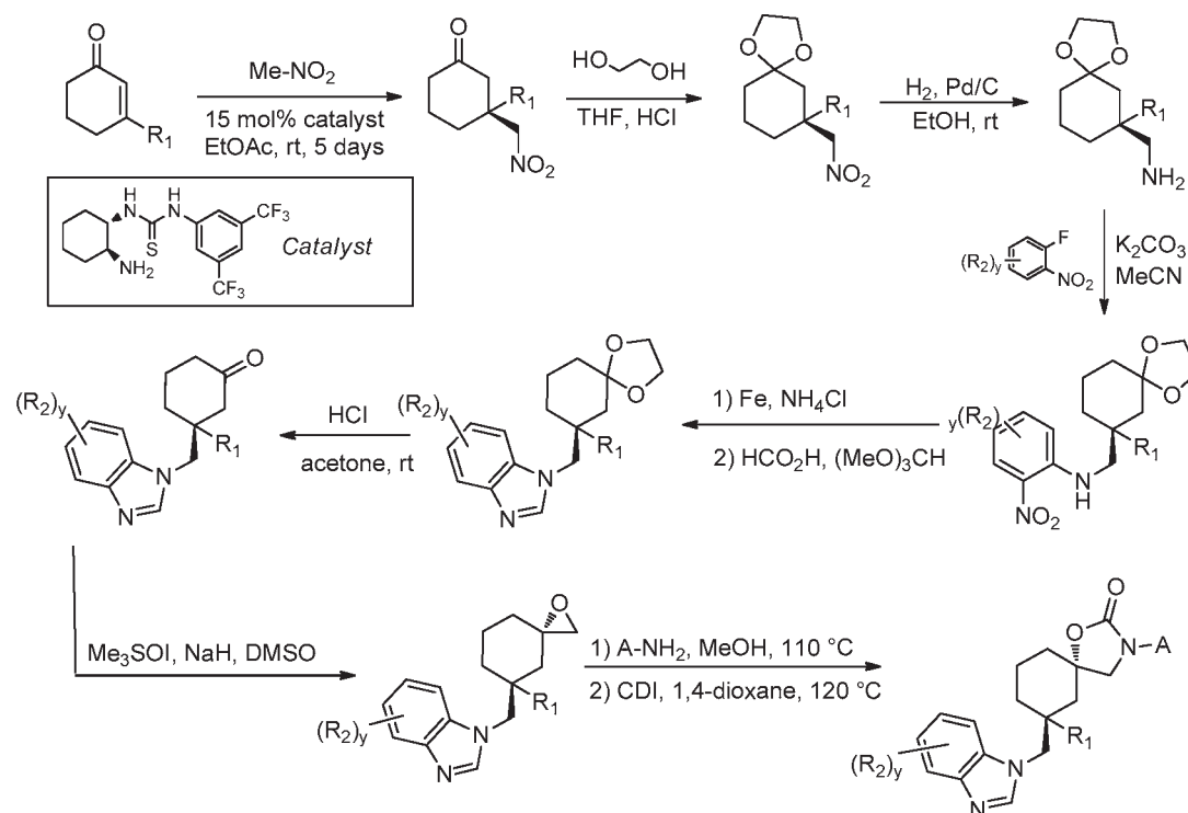
Scheme 4
