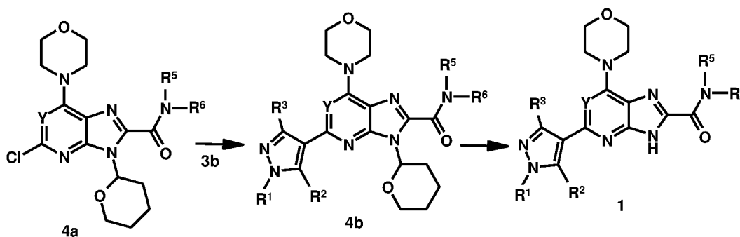
Scheme 4
