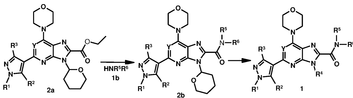
Scheme 2
