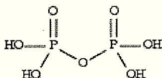
Pyrophosphoric acid
