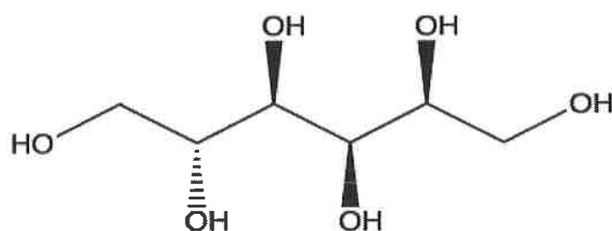
D-sorbitol; and
