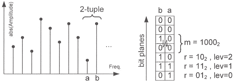
20 Figure 1: Example of a coded pair (2-tuple) of spectral values a and b and their representation as m and r .
