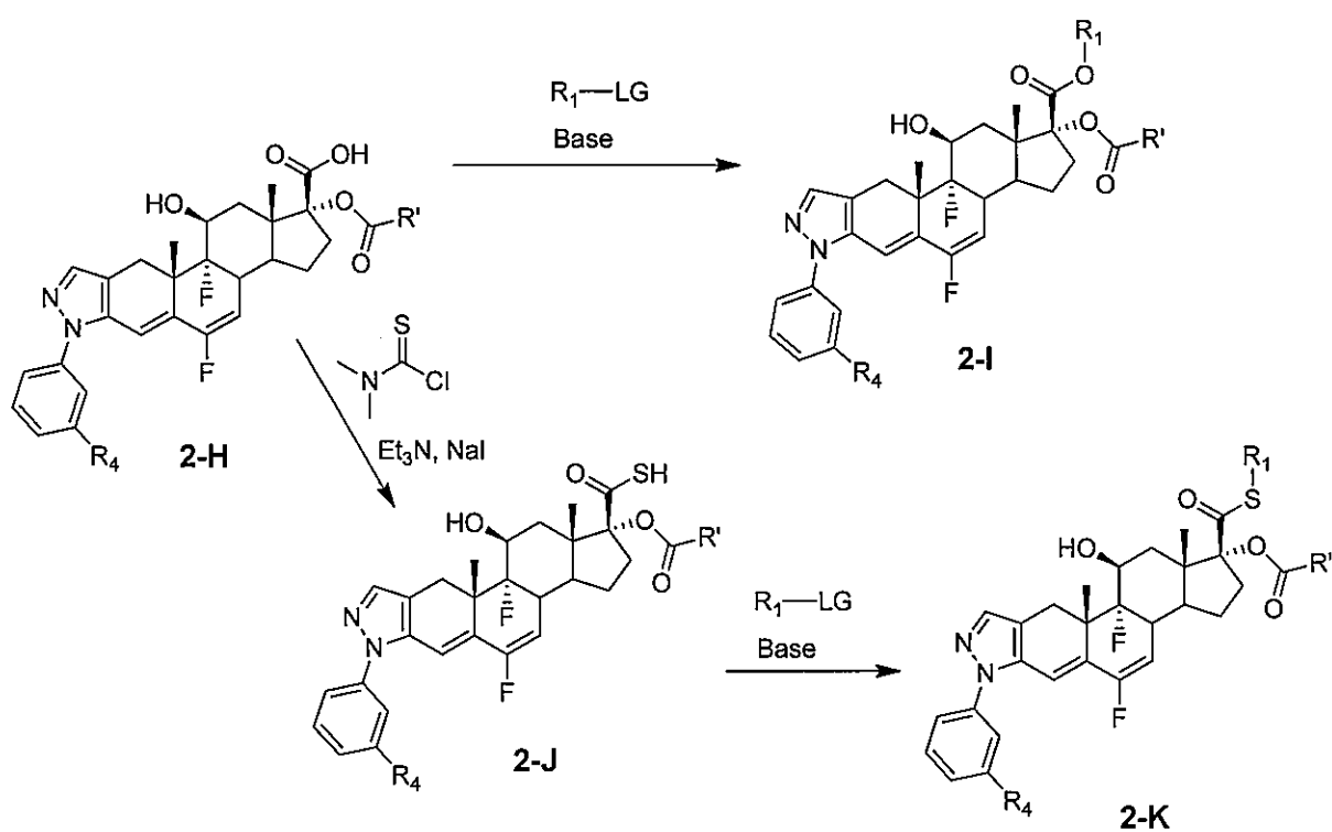
[0145] Scheme 4:
