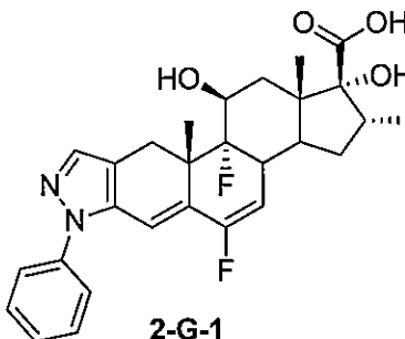
2-G-1
