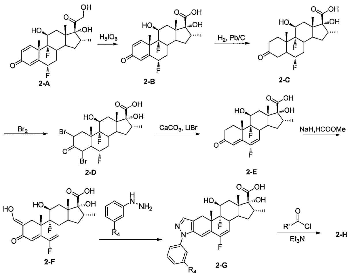
[0144] Scheme 3:
