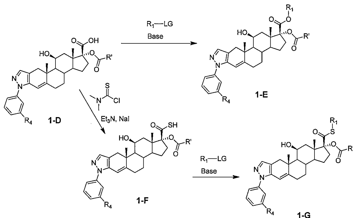
[0141] Scheme 2:
