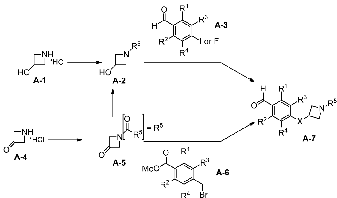
SCHEME A
