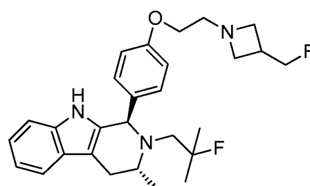
Compound C
