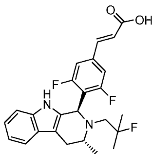
AZD9496
