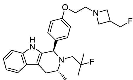
Compound C
