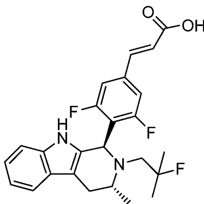
AZD9496
