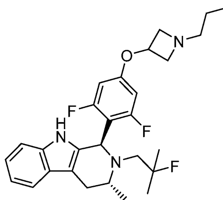
Goodacre Compound 107
