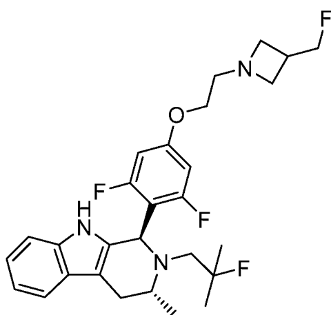
Goodacre Compound 102
