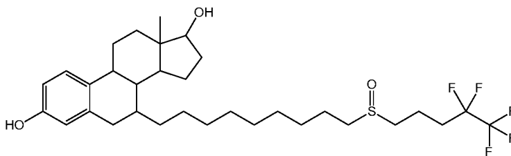
fulvestrant
