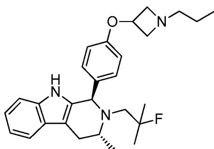
Compound B
