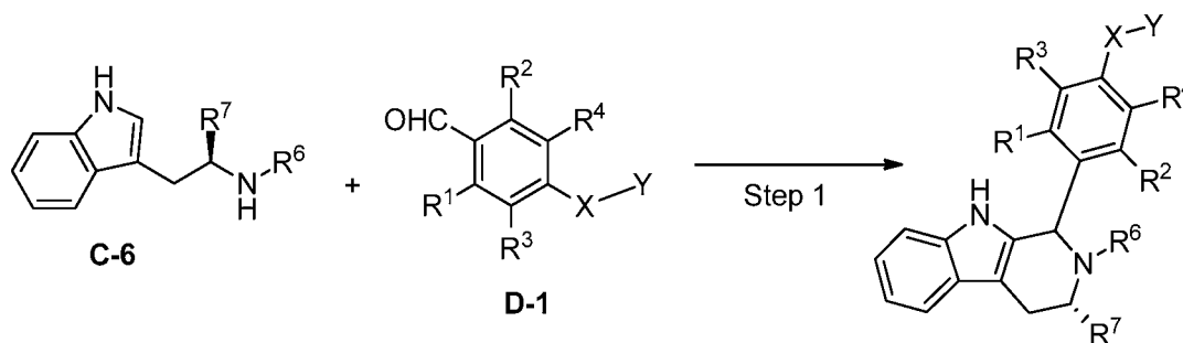
SCHEME D
