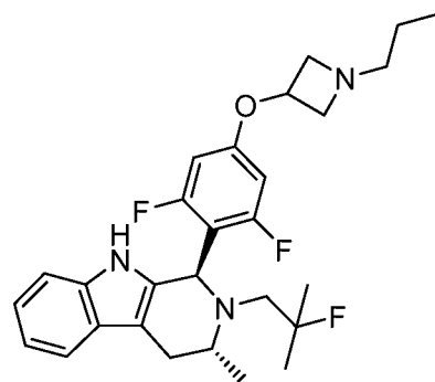
Goodacre Compound 107
