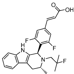
Compound B
