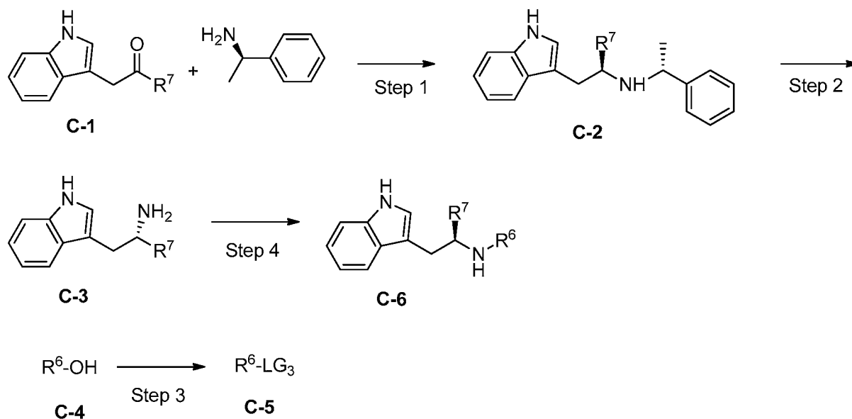
SCHEME C
