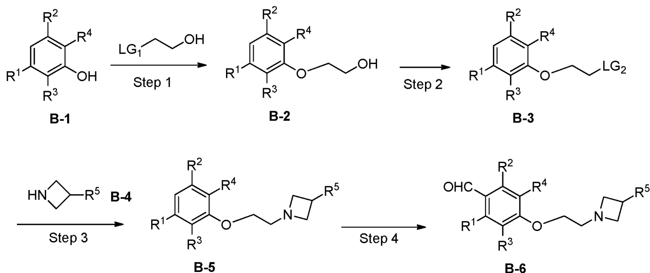
SCHEME B
