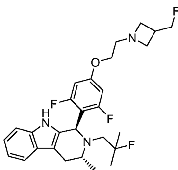
Goodacre Compound 102
