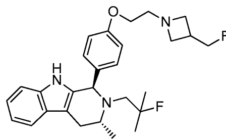
Compound C
