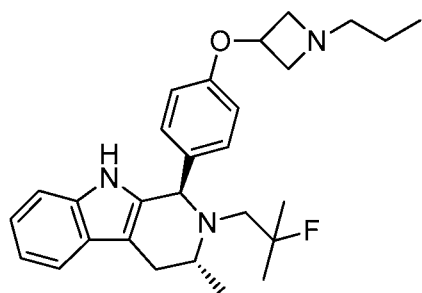
Compound B
