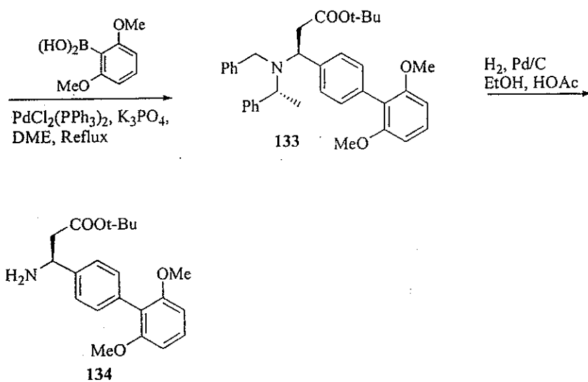
Scheme 33
