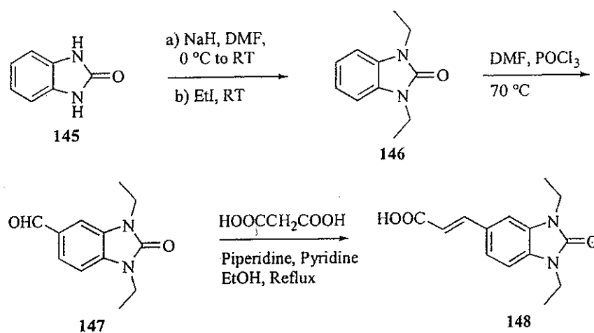
Scheme 35
