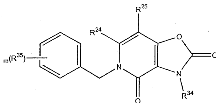
Formula VIII
