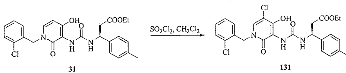
Scheme 32
