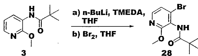
Scheme 7
