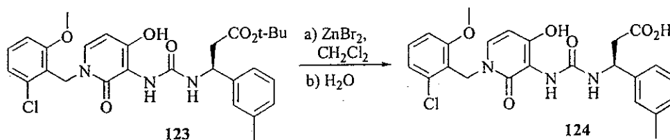
Scheme 28
