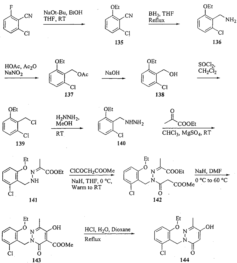
Scheme 34
