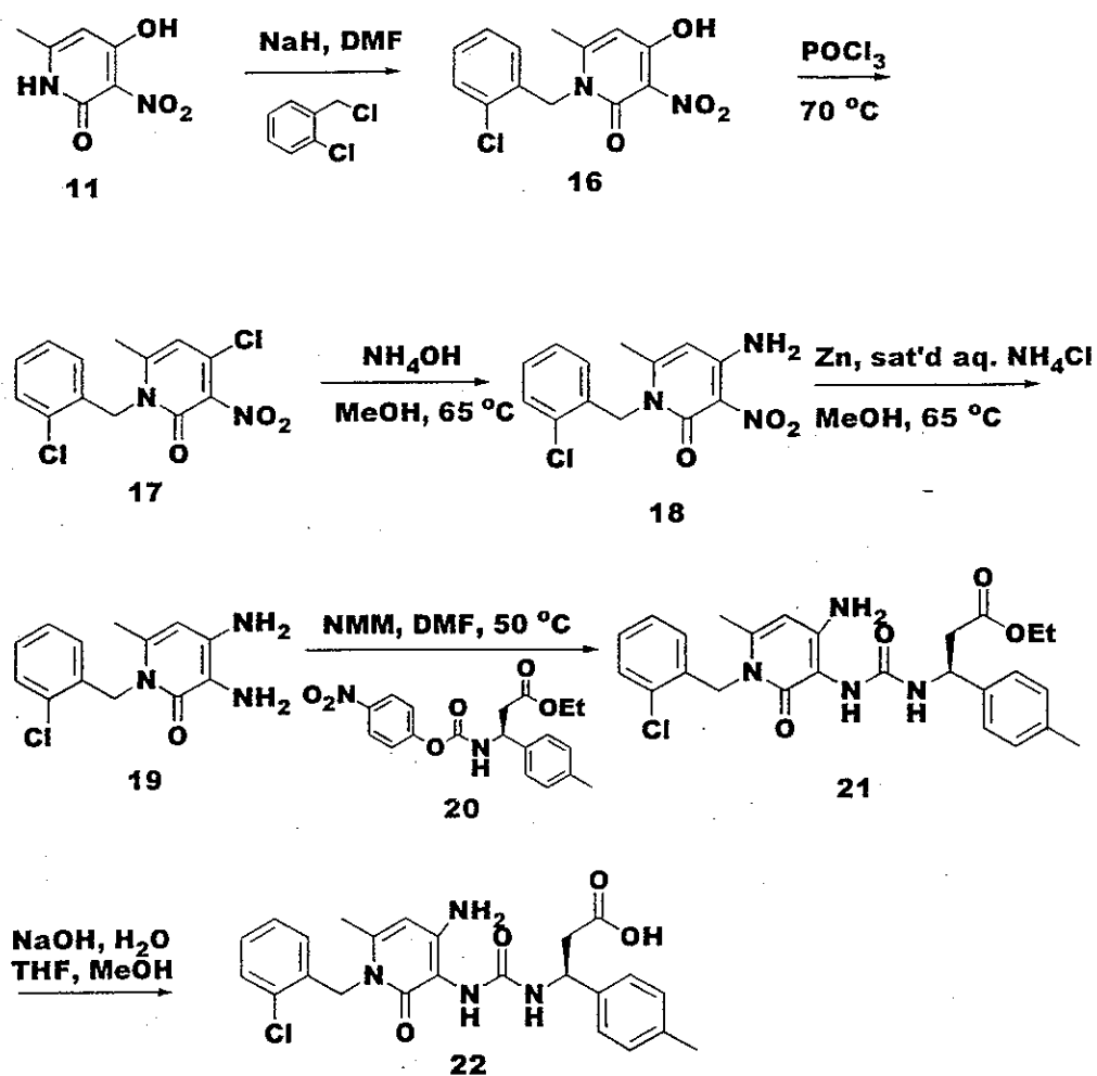
Scheme 3
