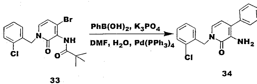
Scheme 9
