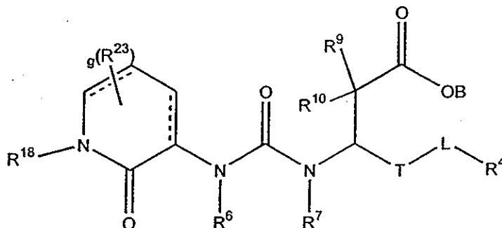
Formula IV
