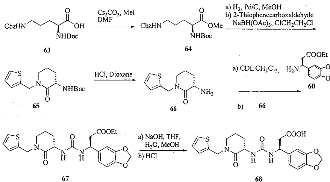
Scheme 16
