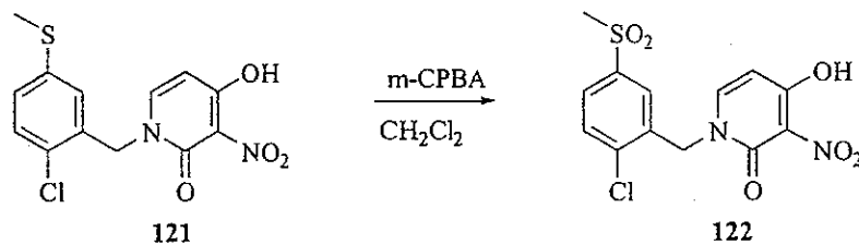
Scheme 27
