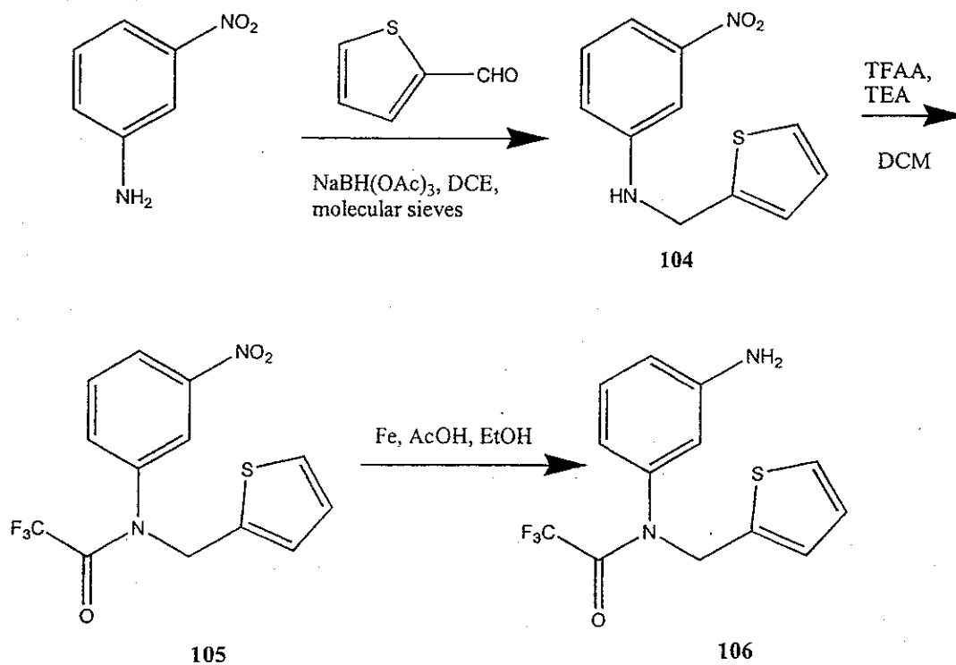
Scheme 21
