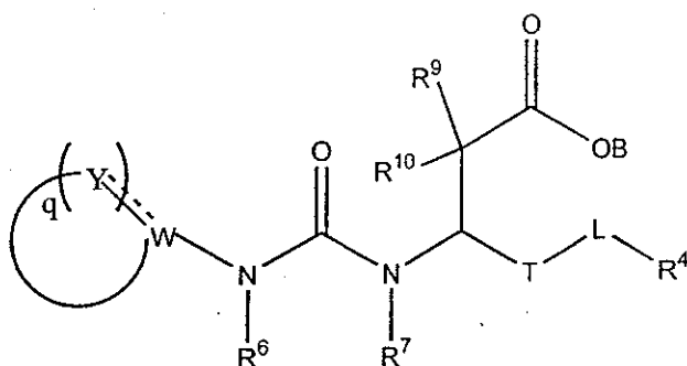
Formula II
