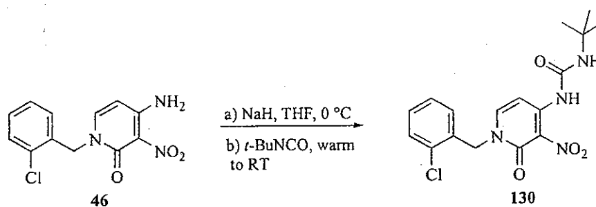
Scheme 31
