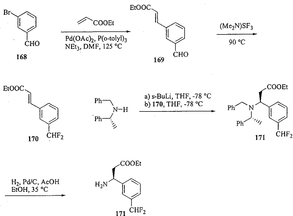
Scheme 42
