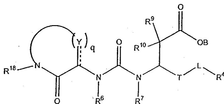
Formula III
