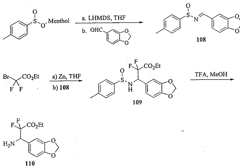
Scheme 22
