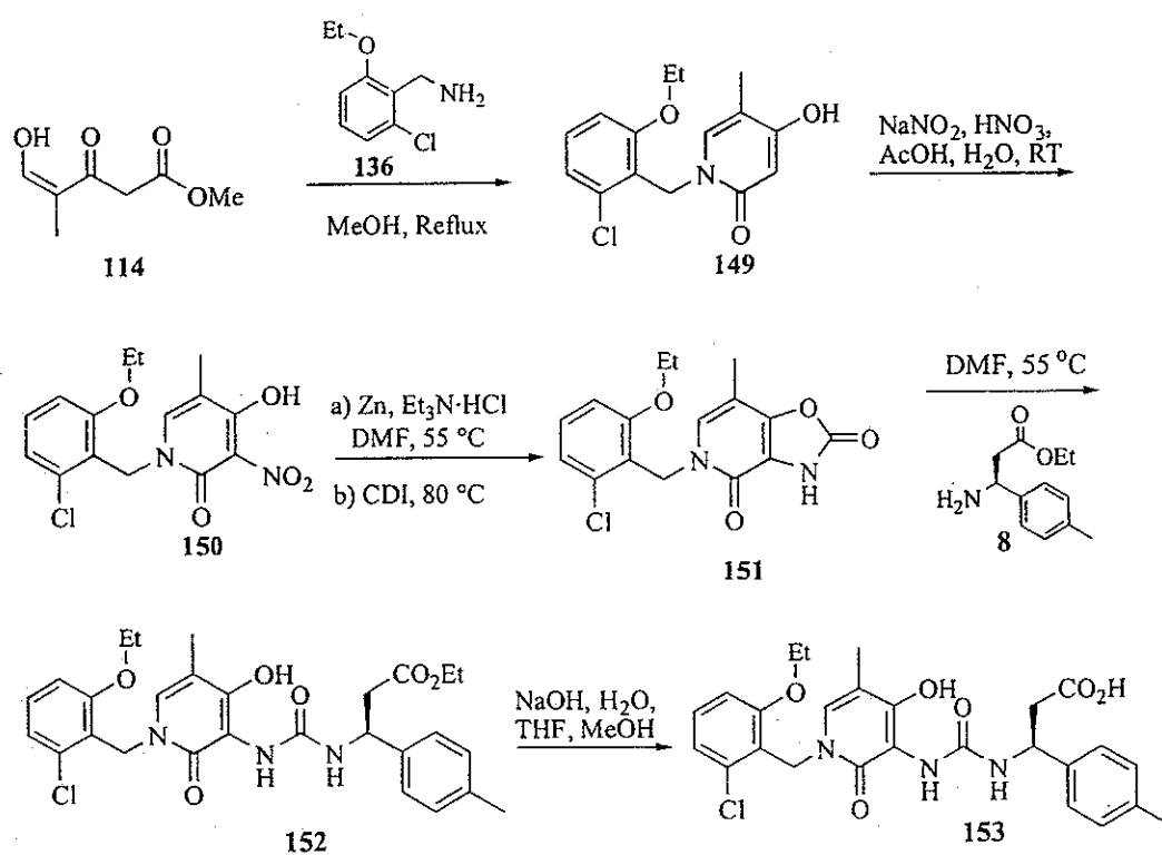
Scheme 36
