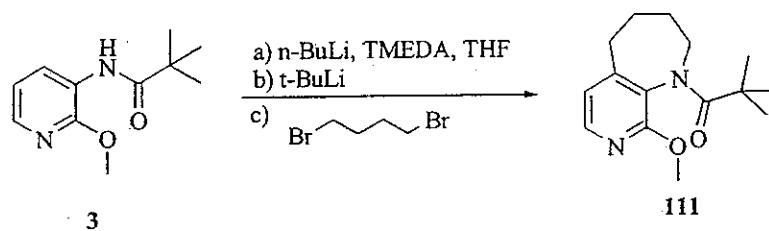
Scheme 23
