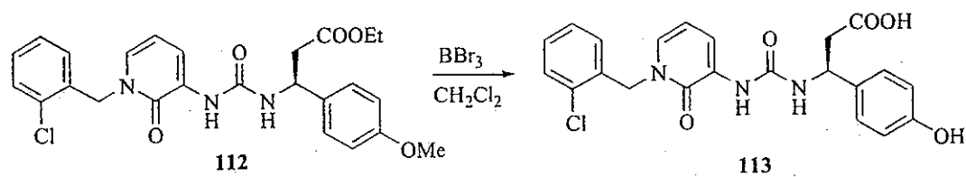
Scheme 23
