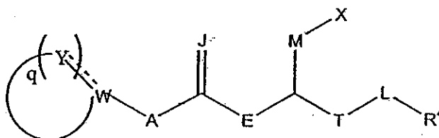
Formula I
