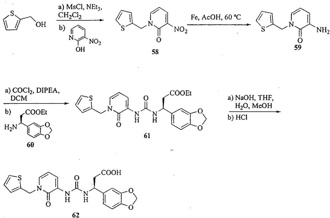
Scheme 15
