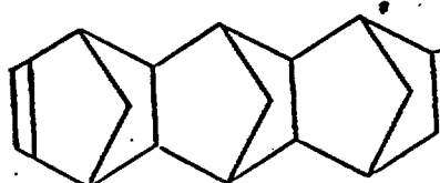
12-Ethylhexacyclo[6,6,1,1 3.6 , 1 10.13 ,0 2.7 ,0 9.14 ]-4-heptadecene
