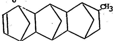
12-Methylhexacyclo[6,6,1,1 3.6 , 1 10.13 ,0 2.7 ,0 9.14 ]-4-heptadecene
