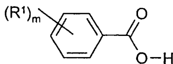
Formula V
