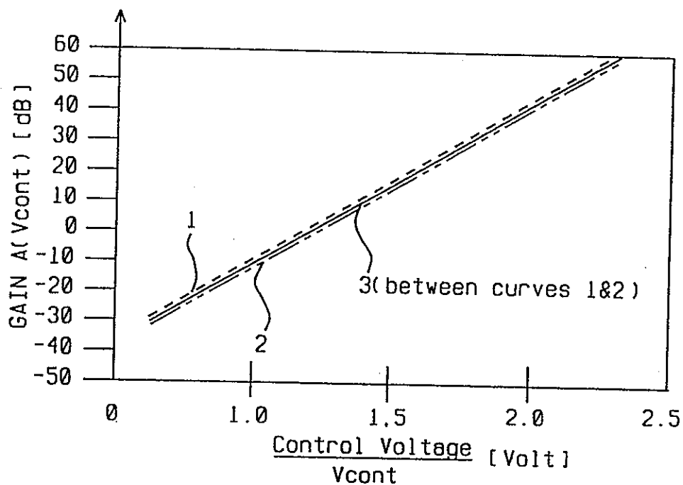
GAIN CONTROL CHARACTERISTICS (FULL COMPENSATION)
