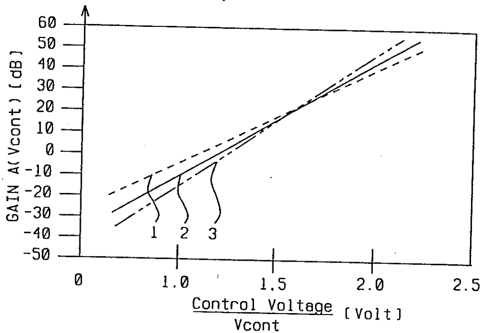
GAIN CONTROL CHARACTERISTICS (PARTIAL COMPENSATION)
