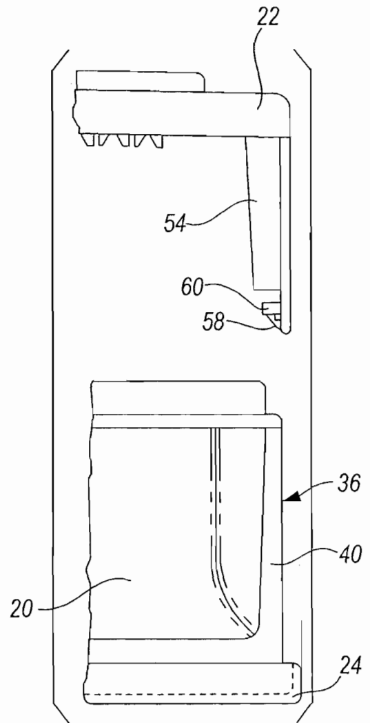
FIG. 4 PRIOR ART
