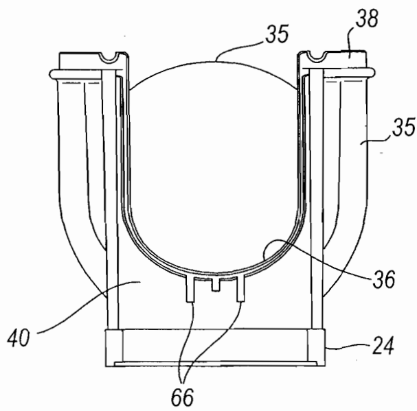
FIG. 6 PRIOR ART
