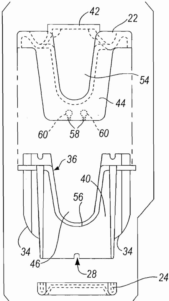
FIG. 3 PRIOR ART
