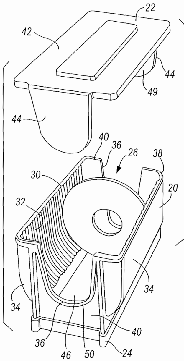
FIG. 1 PRIOR ART
