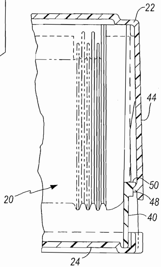
FIG. 2 PRIOR ART
