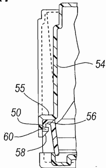
FIG. 5 PRIOR ART
