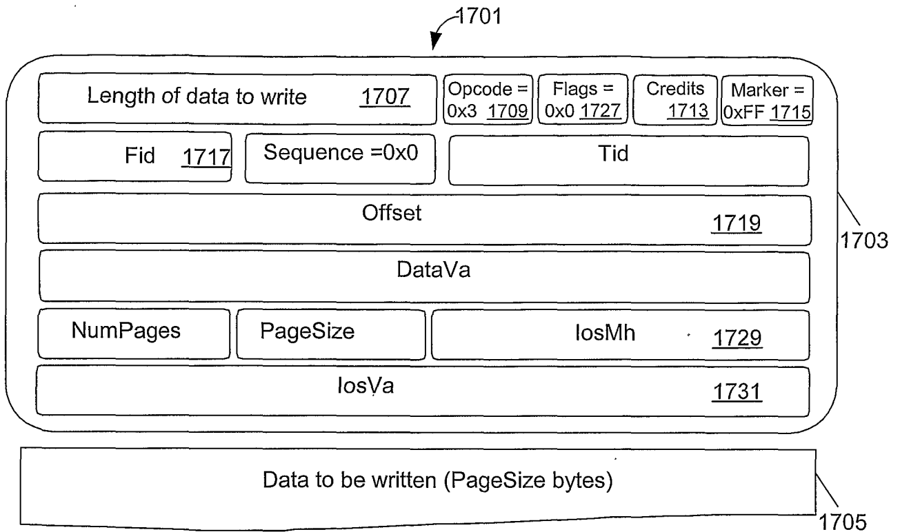
CLIENT VECWRITE MESSAGE, COLLAPSED (POLLING)
