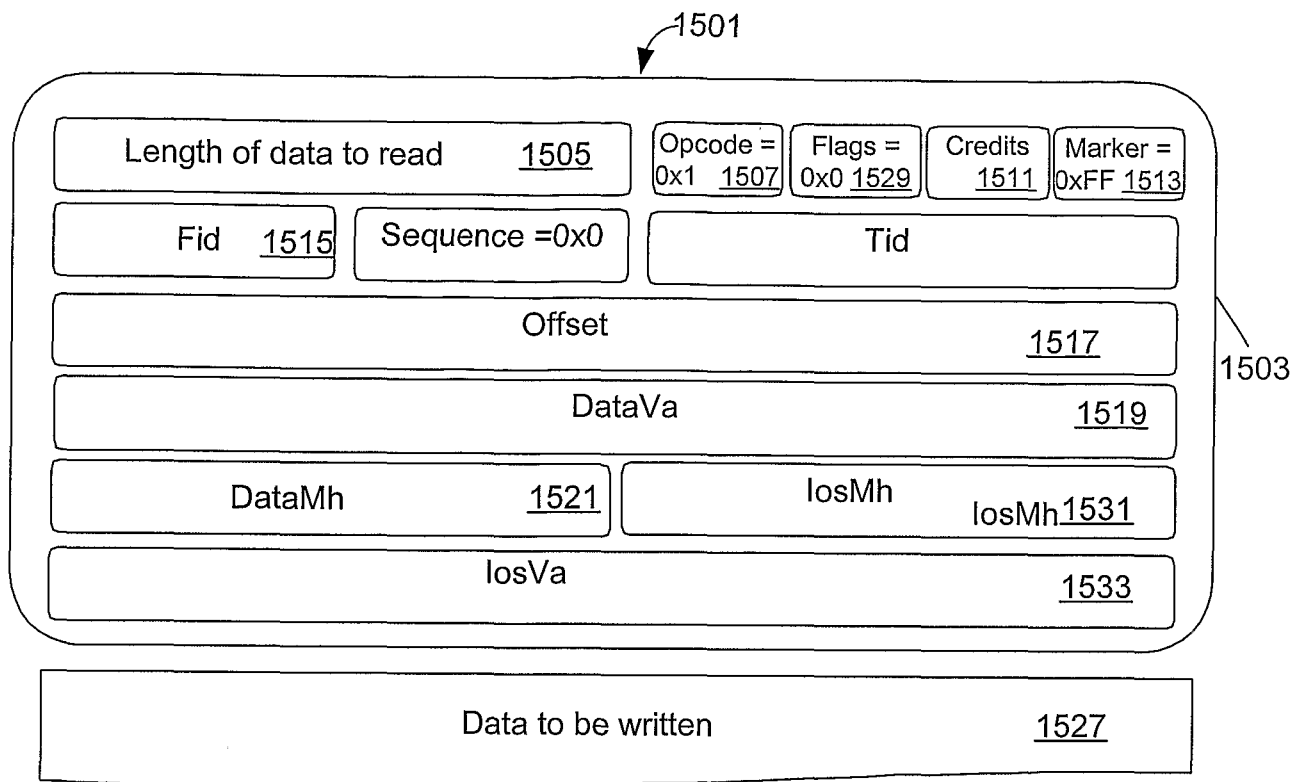
CLIENT WRITE MESSAGE (POLLING)
