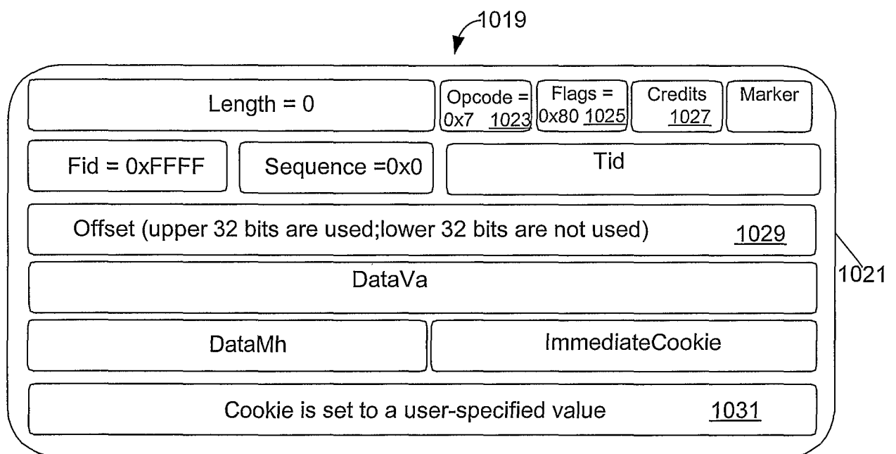
CLIENT-TO-SERVER CREDIT MESSAGE
