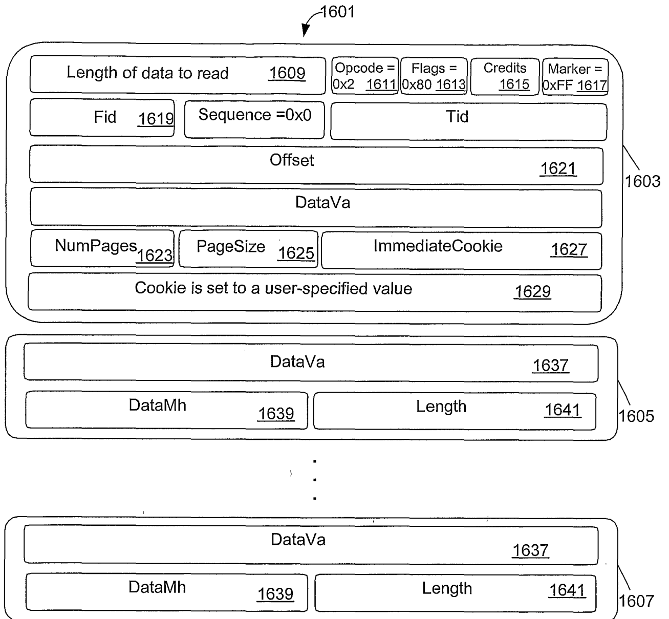
CLIENT VECREAD MESSAGE (NO POLLING)
