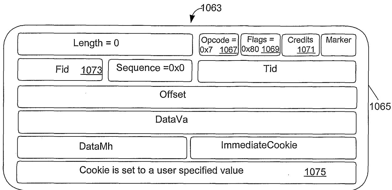
CLIENT CANCEL MESSAGE
