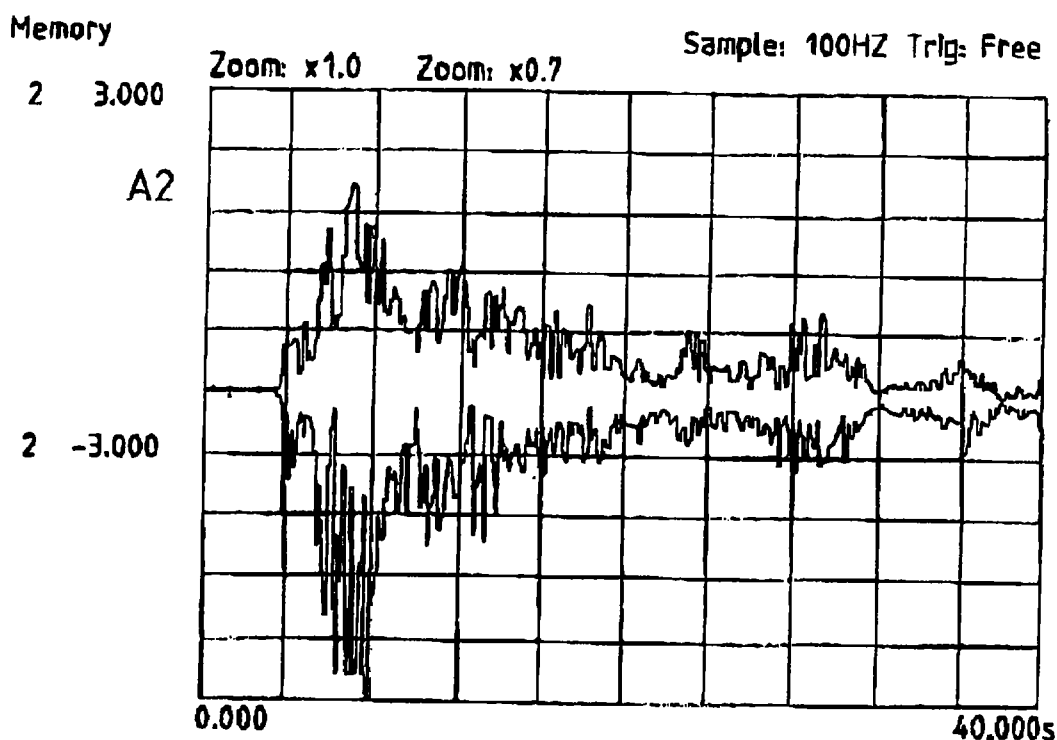
15 Figure 1 Dynamic response of conventional mix - 1100 kg/m 3 density
