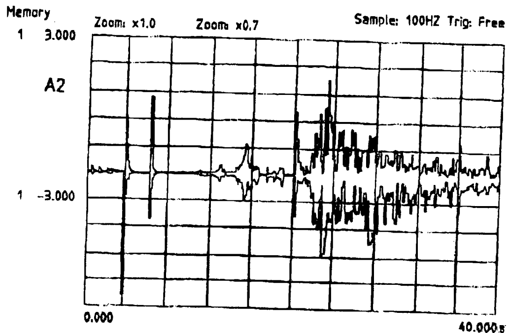
Figure 2 Dynamic response of air-entrained mix - 500 kg/m 3 density
