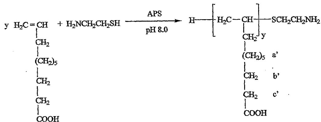
Scheme 3 Synthesis of PUA-NH 2 .
