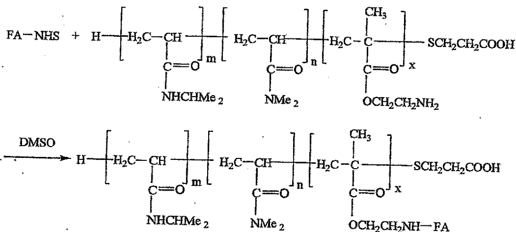
Scheme 2 Synthesis of folate-conjugated P(NIPAAm-co-DMAAm-co-AMA)-COOH.
