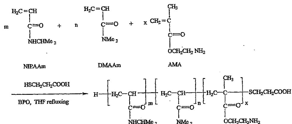
Scheme 1 Synthesis of P(NIPAAm-co-DMAAm-co-AMA)-COOH.
