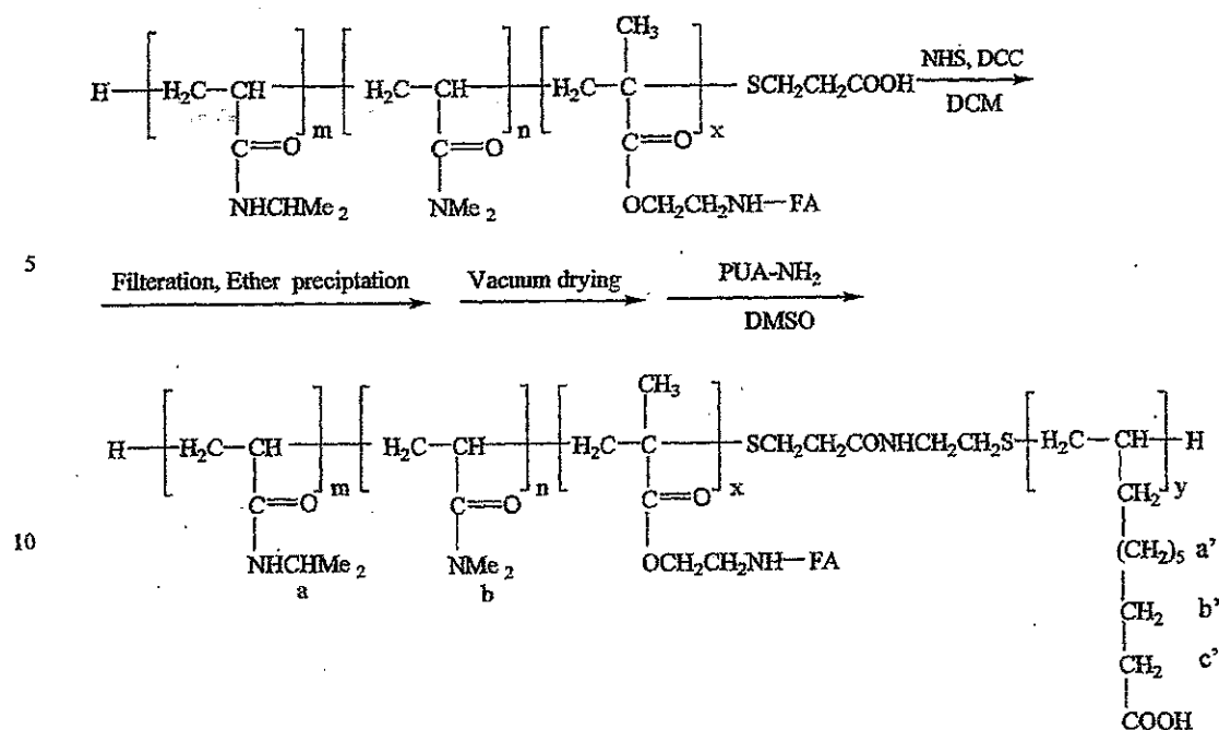
15 Scheme 4 Synthesis of folate-conjugated P(NIPAAm-co-DMAAm-co-AMA)-b-PUA.
