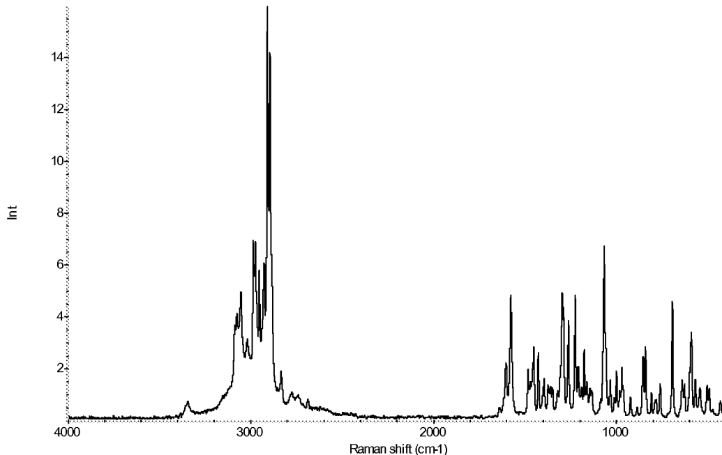
Raman spectrum (1).
