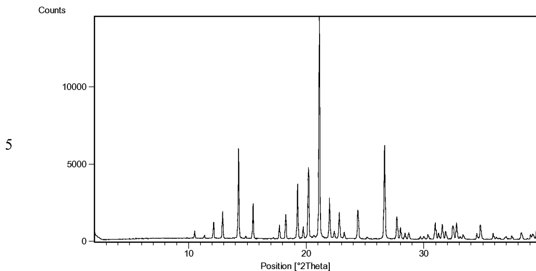
(XRPD pattern 1).
