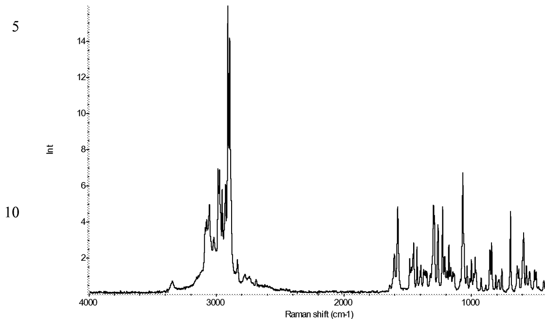
Raman spectrum (1).
