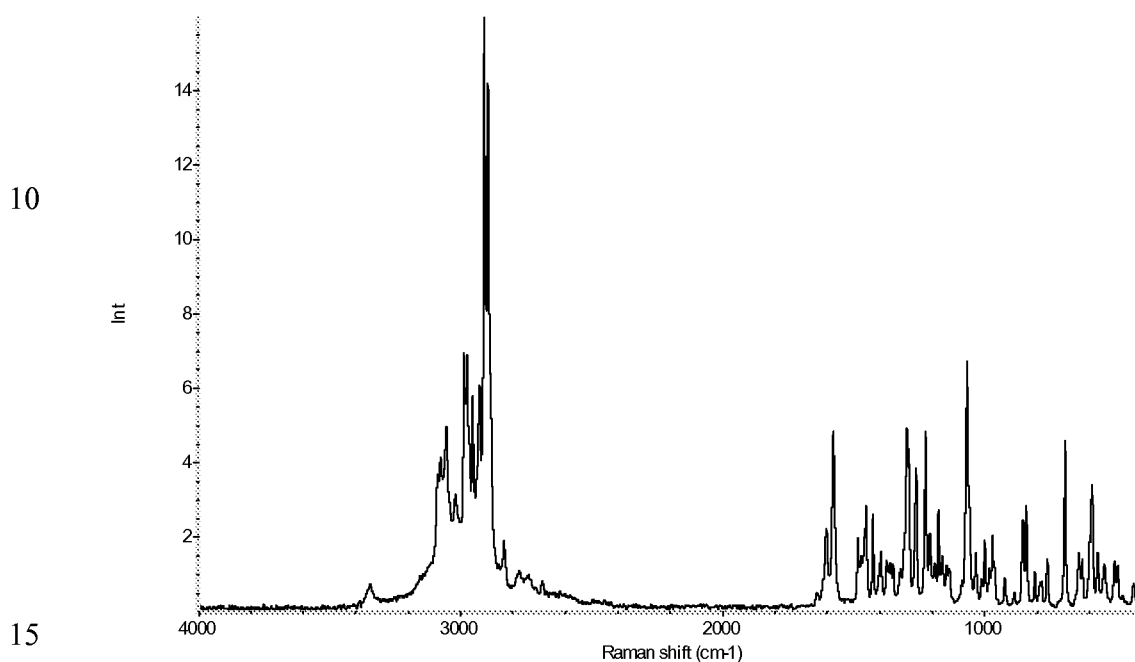
Raman spectrum (1).
