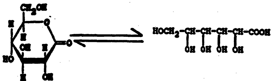
Glucono-delta-lactone (GDL)
