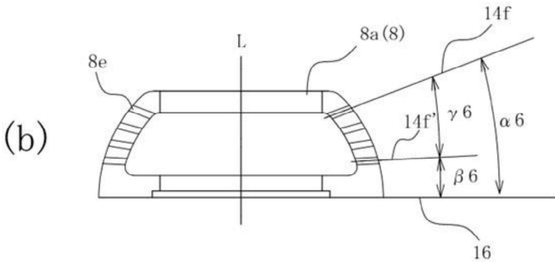
F-F CROSS SECTION
