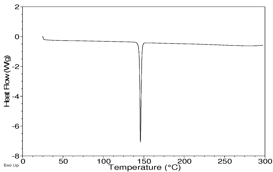
Figure 4: DSC Thermogram of Form B of 7-Fluoro-1-isopropyl-3-methyl-8-[6-[3-(1- 5 piperidyl)propoxy]-3-pyridyl]imidazo[4,5-c]quinolin-2-one
