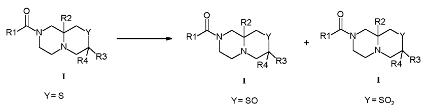
Scheme 8
