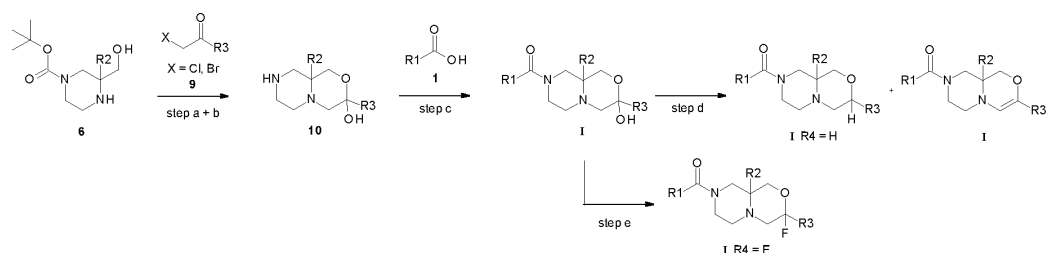
Scheme 3b
