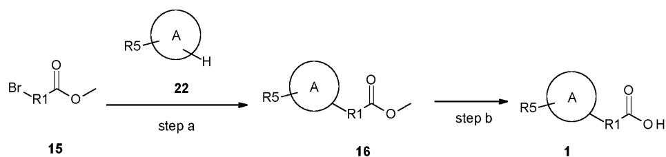
Scheme 9d
