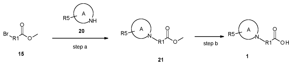
Scheme 9c
