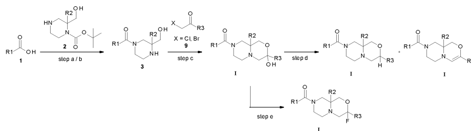
Scheme 3a
