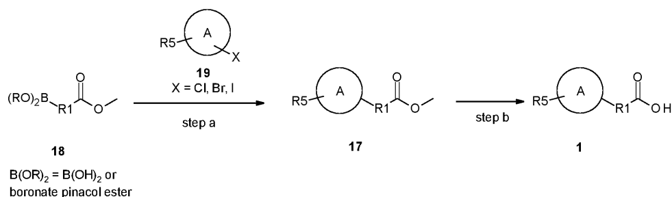
Scheme 9b
