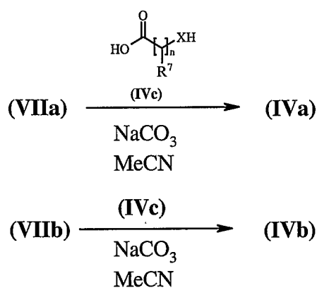
Scheme 2
