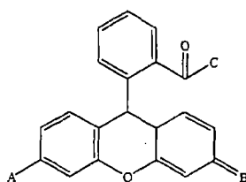
General structure of rhodamine family
