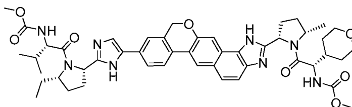
Methyl[(1S)-2-[(2S,5S)-2-(9-{2-[(2S,5S)-5-ethyl-1-[(2S)-2[(methoxycarbonyl)amino]-3-methylbutanoyl]pyrrolidin-2-yl]-1H-imidazol-5-yl]-1,11dihydroisochromeno [4',3':6,7]naphtho[1,2-d]imidazol-2-yl)-5-methylpyrrolidin-1-yl]-2-oxo-1(tetrahydro-2H-pyran-4-yl)ethyl]carbamate
