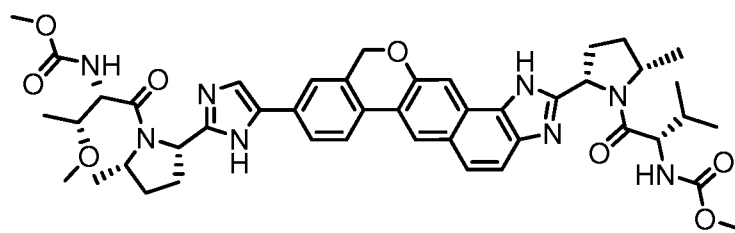
methyl {(2S)-1-[(2S,4S)-2-(5-{2-[(2S,5S)-1-[(2S,3R)-3-methoxy-2-[(methoxycarbonyl)amino]butanoyl]-5-methylpyrrolidin-2-yl]-1,11-dihydroisochromeno[4',3':6,7]naphtho[1,2-d]imidazol-9-yl)-1H-imidazol-2-yl]-5-methylpyrrolidin-1-yl]-3-methyl-1-oxobutan-2-yl}carbamate
