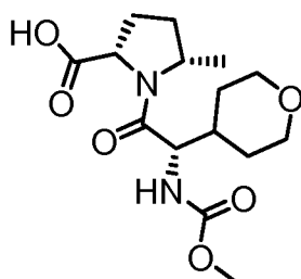
(2S,5S)-1-((S)-2-(methoxycarbonylamino)-2-(tetrahydro-2H-pyran-4-yl)acetyl)-5-methyl pyrrolidine-2-carboxylic acid
