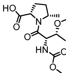
(2S,5S)-1-((2S,3R)-3-methoxy-2-(methoxycarbonylamino)butanoyl)-5-methylpyrrolidine-2-carboxylic acid
