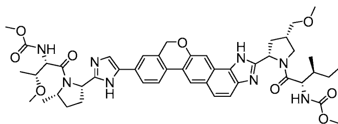
methyl{(2S,3S)-1-[(2S,4S)-2-(9-{2-[(2S,5S)-1-{(2S,3R)-3-methoxy-2-[(methoxy carbonyl)amino]butanoyl}-5-methylpyrrolidin-2-yl]-1H-imidazol-5-yl}-1,11-dihydroisochromeno[4',3':6,7]naphtho[1,2-d]imidazol-2-yl)-4-(methoxymethyl)pyrrolidin-1-yl]-3-methyl-1-oxopentan-2-yl} carbamate
