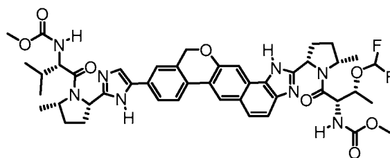
methyl {(2S)-1-[(2S,5S)-2-(5-{2-[(2S,5S)-1-[(2S,3R)-3-(difluoromethoxy)-2-[(methoxycarbonyl)amino]butanoyl]-5-methylpyrrolidin-2-yl]-1,11-dihydroisochromeno[4',3':6,7]naphtho[1,2-d]imidazol-9-yl)-1H-imidazol-2-yl]-5-methylpyrrolidin-1-yl]-3-methyl-1-oxobutan-2-yl} carbamate
