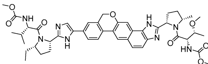
methyl{(2S,3R)-1-[(2S,5S)-2-(9-{2-[(2S,5S)-5-ethyl-1-{(2S)-2-[(methoxycarbonyl) amino]-3-methylbutanoyl}pyrrolidin-2-yl]-1H-imidazol-5-yl}-1,11-dihydroisochromeno[4',3':6,7]naphtho[1,2-d]imidazol-2-yl)-5-methylpyrrolidin-1-yl]-3-methoxy-1-oxobutan-2-yl} carbamate
