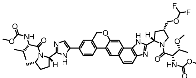
methyl [(2S,3R)-1-[(2S,4S)-4-[(difluoromethoxy)methyl]-2-[9-(2-[(2S,5S)-1-[N-(methoxycarbonyl)-L-valyl]-5-methylpyrrolidin-2-yl]-1H-imidazol-5-yl)-1,11-dihydroisochromeno[4',3':6,7]naphtho[1,2-d]imidazol-2-yl]pyrrolidin-1-yl]-3-methoxy-1-oxobutan-2-yl]carbamate
