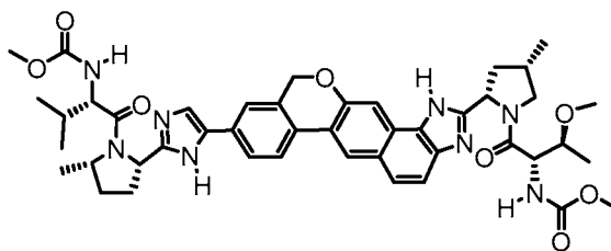
methyl {(2S)-1-[(2S,5S)-2-(5-{2-[(2S,4S)-1-{(2S,3S)-3-methoxy-2-[(methoxycarbonyl)amino]butanoyl}-4-methylpyrrolidin-2-yl]-1,11-dihydroisochromeno[4',3':6,7]naphtho[1,2-d]imidazol-9-yl}-1H-imidazol-2-yl)-5-methylpyrrolidin-1-yl]-3-methyl-1-oxobutan-2-yl}carbamate
