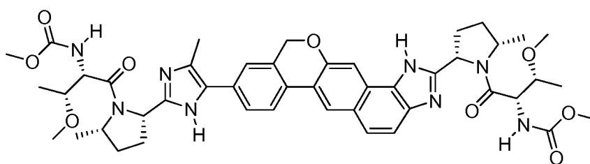
methyl [(2S,3R)-3-methoxy-1-{(2S,5S)-2-[9-(2-{(2S,5S)-1-[N-(methoxycarbonyl)-O-methyl-L-threonyl]-5-methylpyrrolidin-2-yl)-4-methyl-1H-imidazol-5-yl]-1,11-dihydroisochromeno[4',3':6,7]naphtho[1,2-d]imidazol-2-yl]-5-methylpyrrolidin-1-yl}-1-oxobutan-2-yl]carbamate
