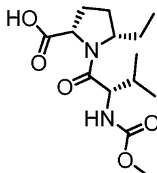
(2S,5S)-5-ethyl-1-((S)-2-(methoxycarbonylamino)-3-methylbutanoyl)pyrrolidine-2-carboxylic acid
