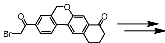
3-(2-bromoacetyl)-10,11-dihydro-5H-dibenzo[c,g]chromen-8(9H)-one
