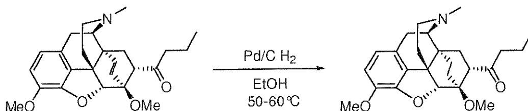
20-ethylthevinone (2)
