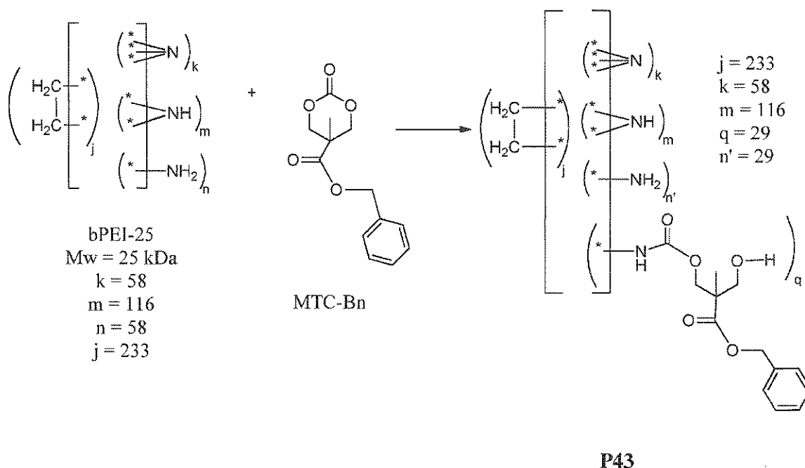
Scheme 7.
