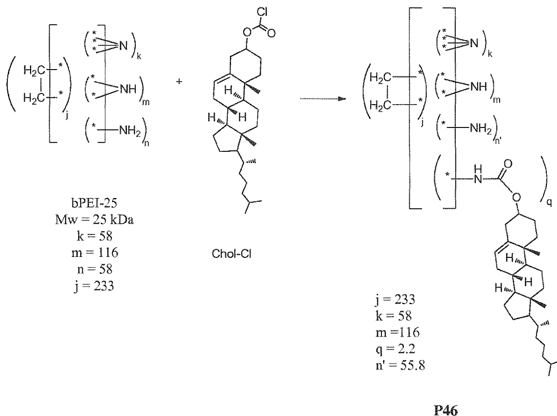
Scheme 11.
