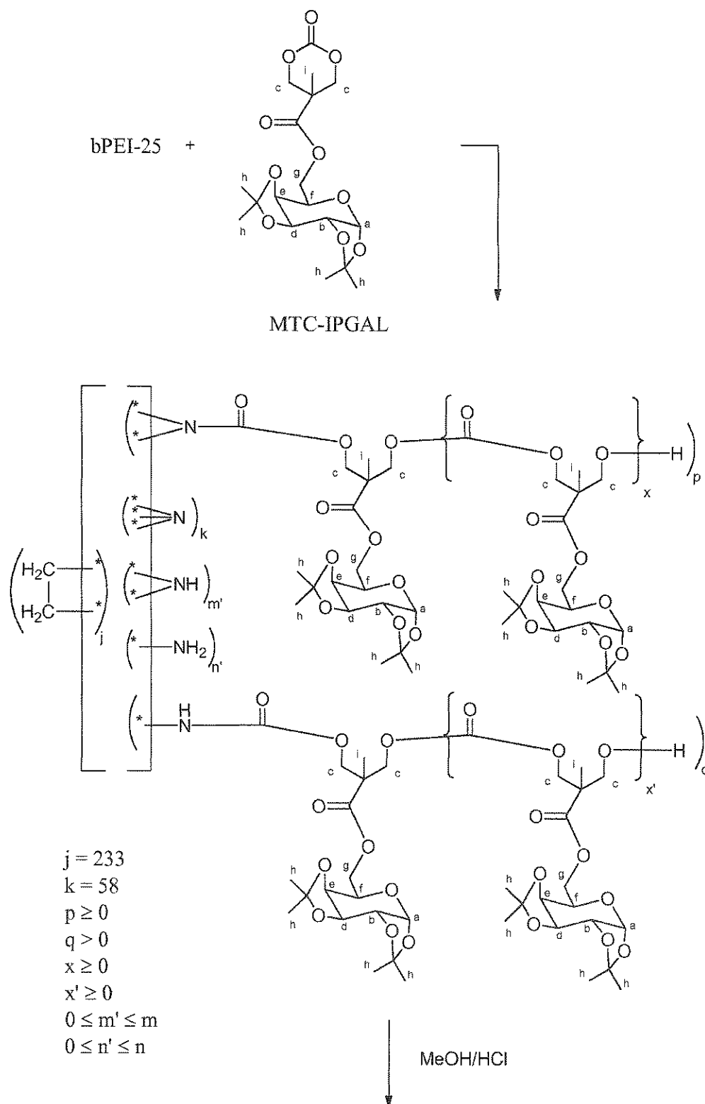
Scheme 4.
