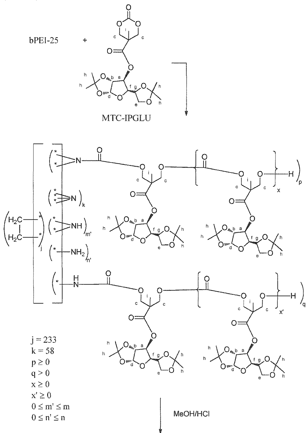
Scheme 3.
