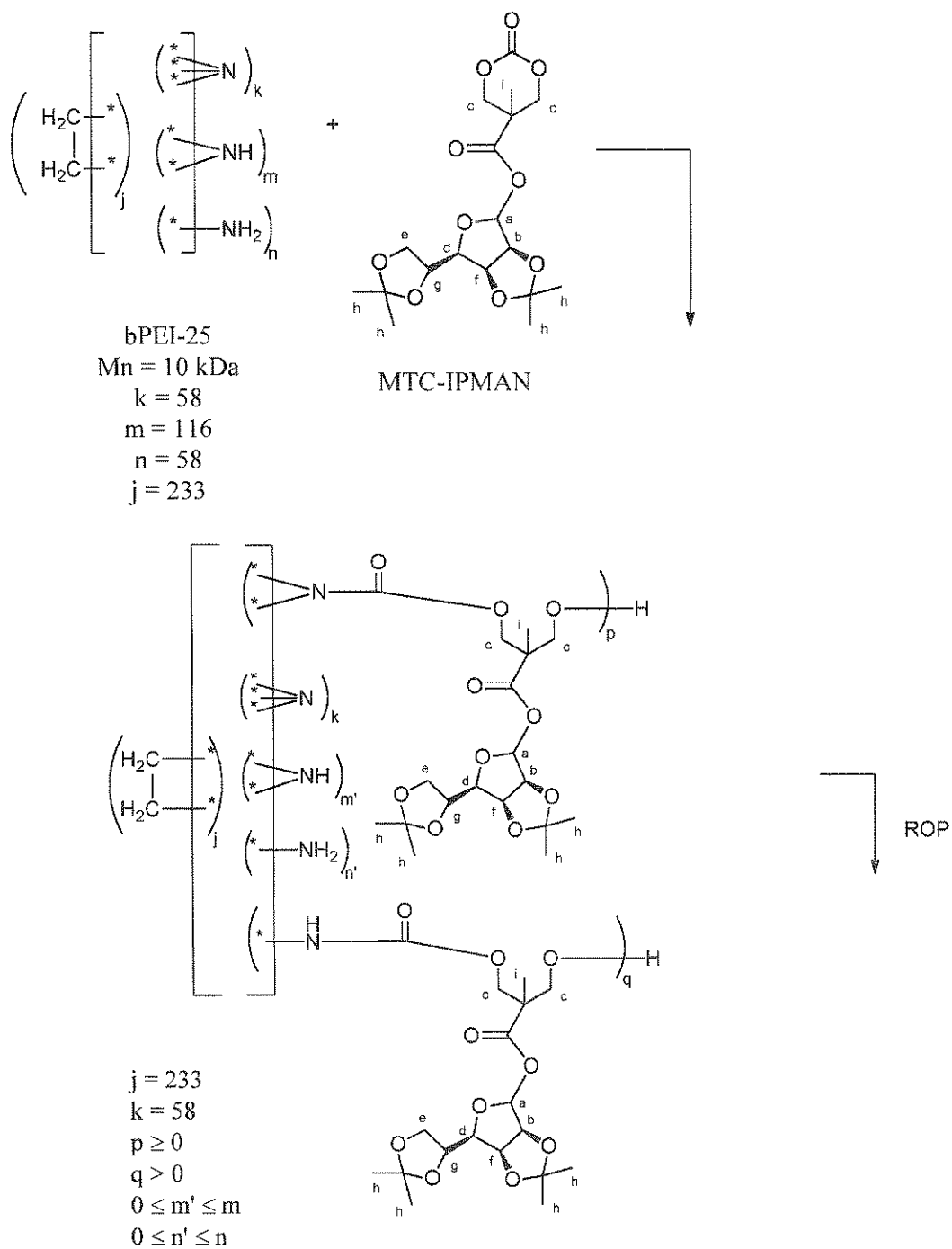
Scheme 2.
