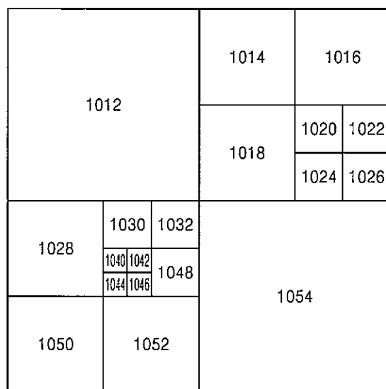
CODING UNIT (1010)
