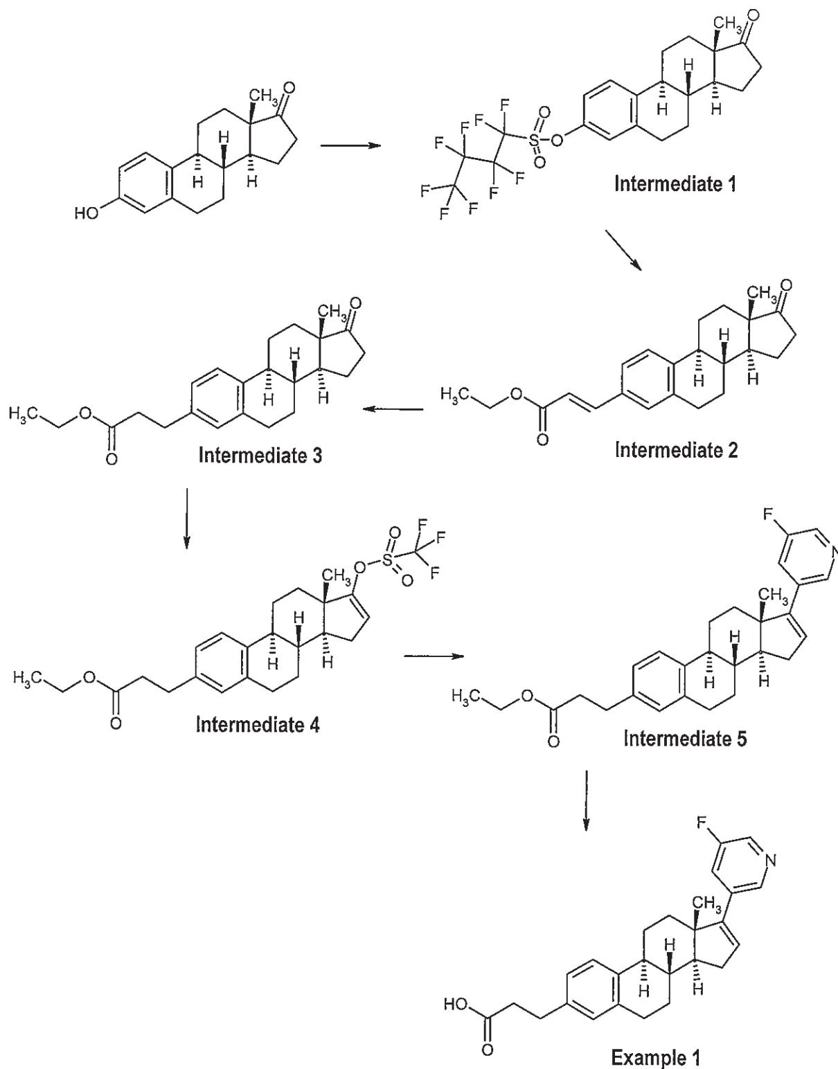
Synthesis scheme 1
