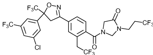
Compound 99
