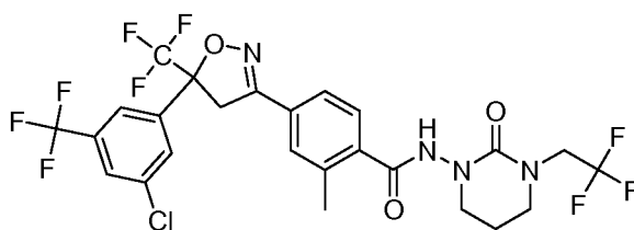
Compound 70
