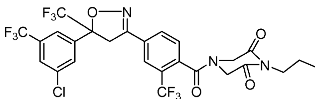
Compound 95
