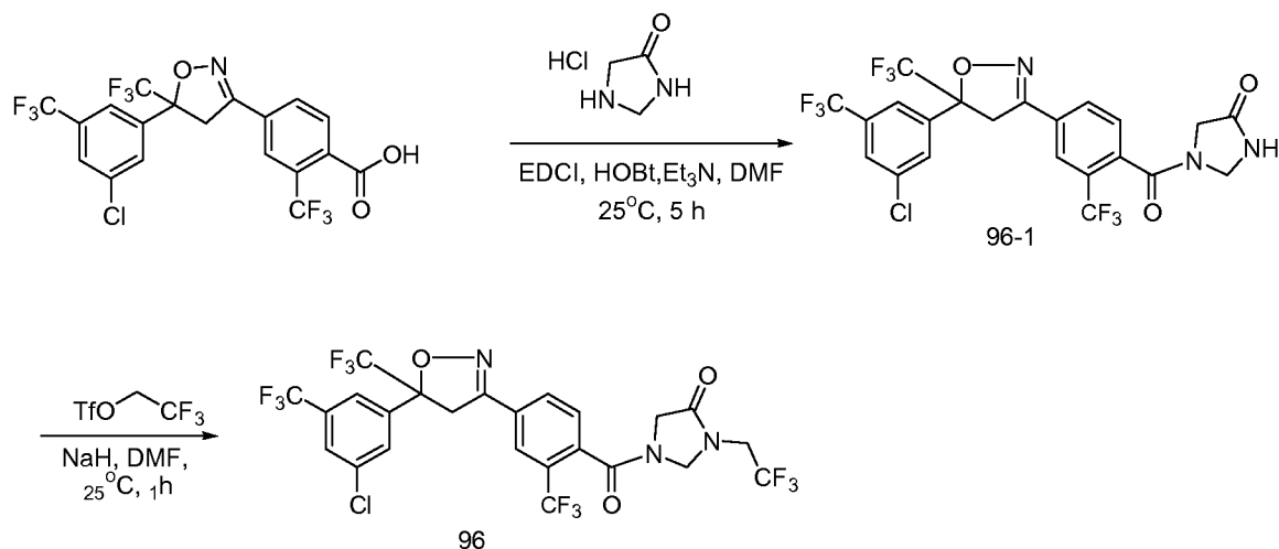
Scheme 11
