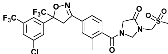
Compound 114
