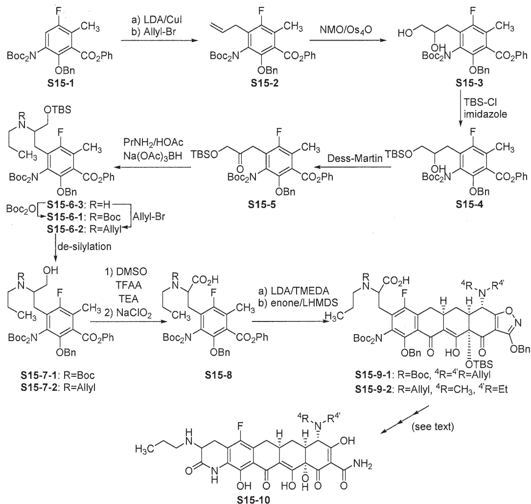
Scheme 15
