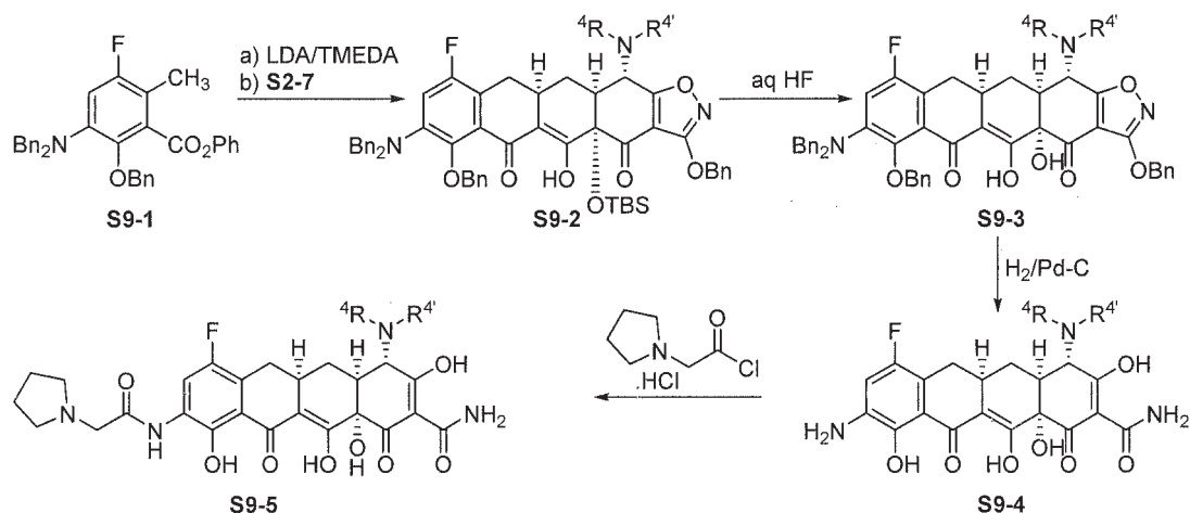
Scheme 9
