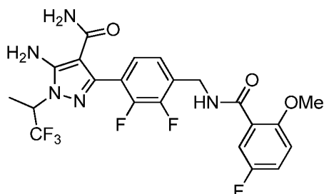
5-Amino-3-(4-bromo-2,3-difluoro-phenyl)-1-(2,2,2-trifluoro-1-methyl-ethyl)pyrazole-4-carbonitrile
