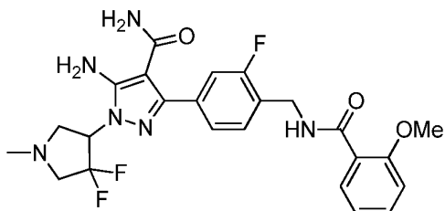
5-Amino-1-(4,4-difluoro-1-methyl-pyrrolidin-3-yl)-3-[3-fluoro-4-[(2-methoxybenzoyl)amino]methyl]phenyl]pyrazole-4-carboxamide
