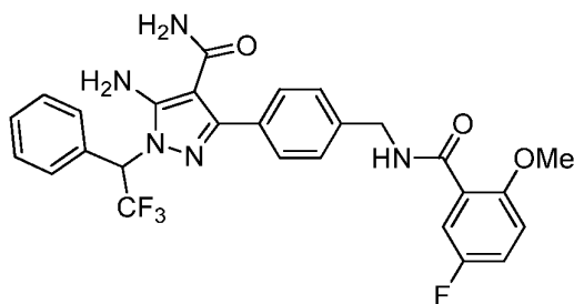
N-[(2,2,2-Trifluoro-1-phenyl-ethylidene)amino]benzamide
