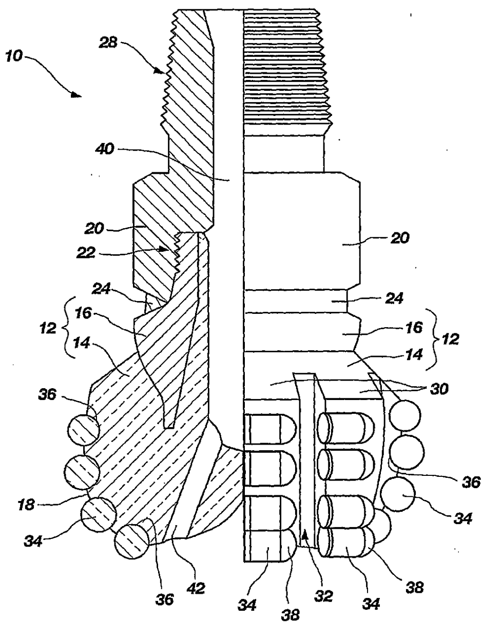
FIG. 1 (PRIOR ART)
