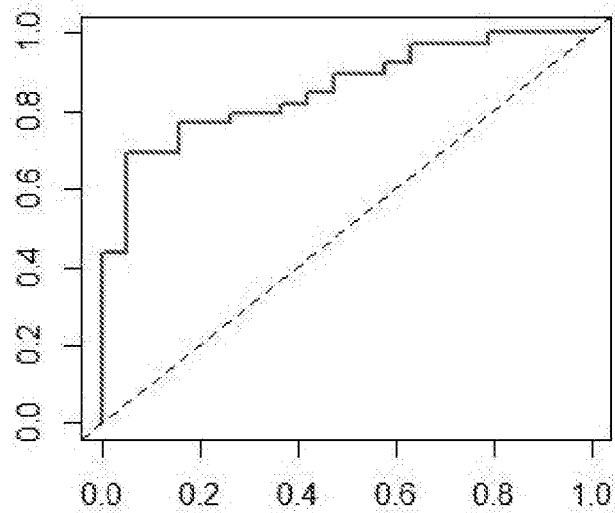
Normal vs other (AUC: 0.856 )
