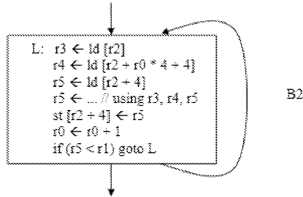
Pseudo Code B: Pseudo code region to be optimized
