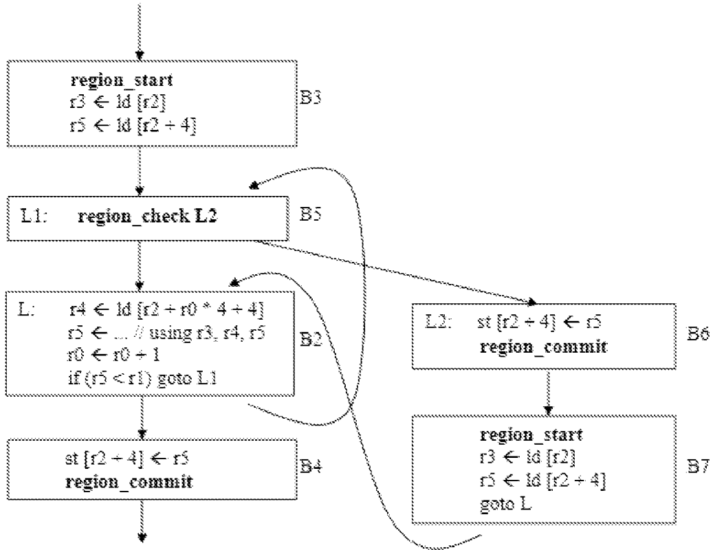
Pseudo Code E: Code region after optimization
