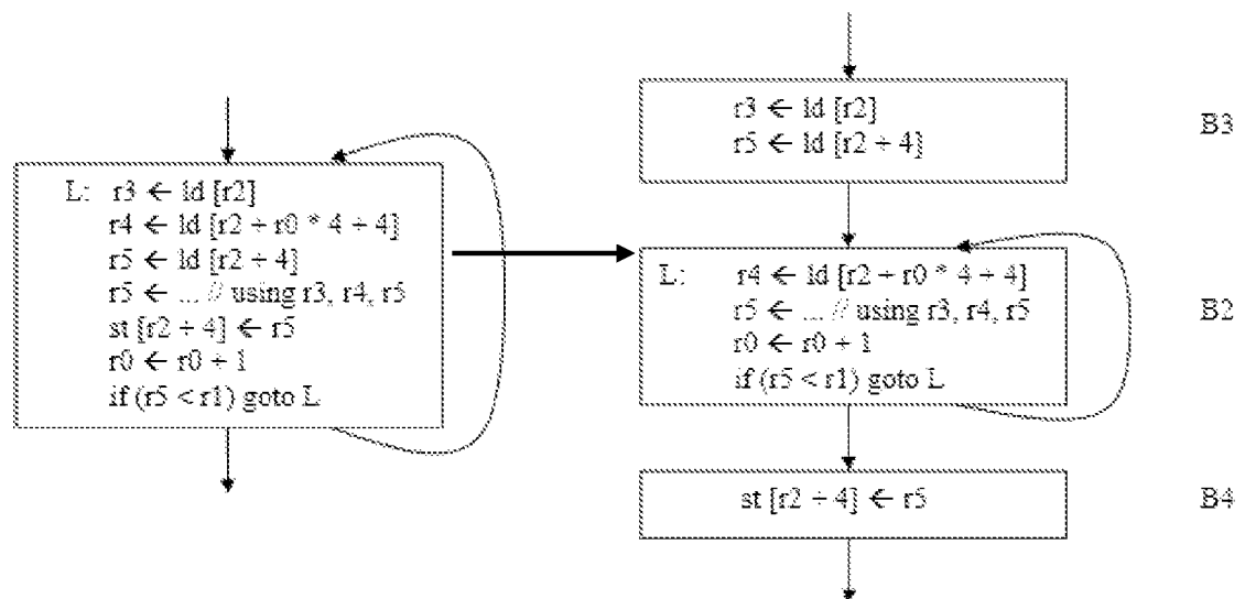
Pseudo Code A: An embodiment of single threaded code optimization
