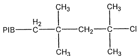
PIB tert-Chloride
