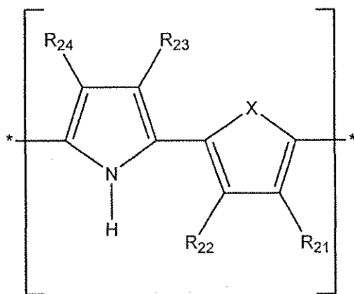
Formula III
