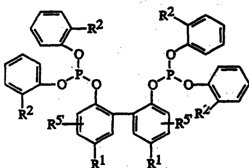
Formula I
