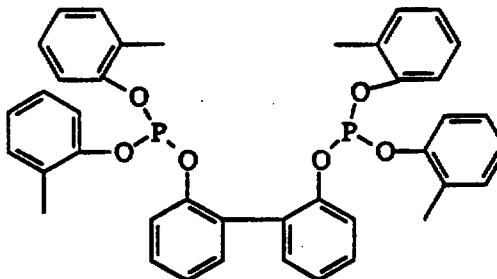
Ligand "A3"
