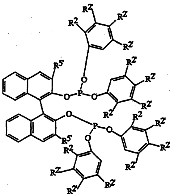
Formula V
