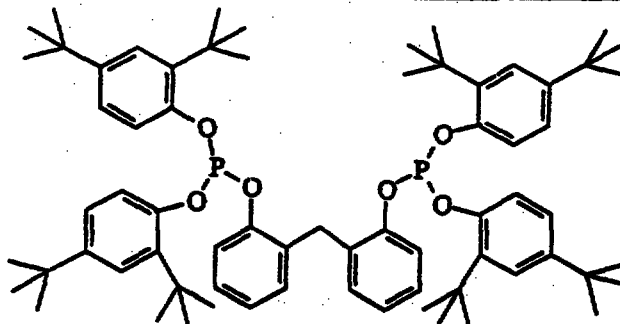
Ligand "J2"
