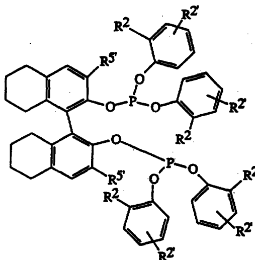
Formula VII
