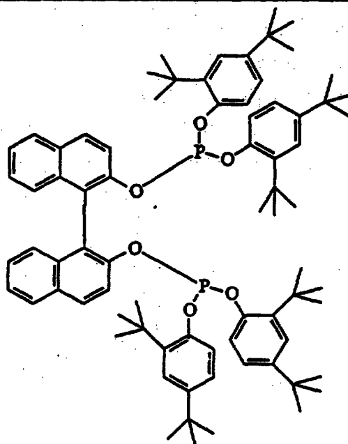
Ligand "P"
