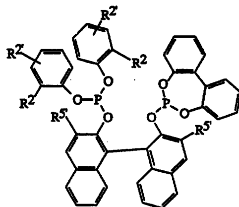
Formula IV
