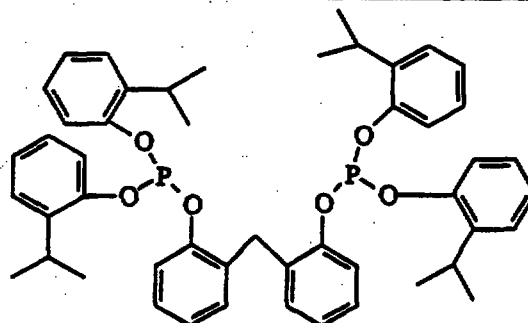
Ligand "C"
