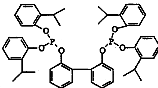
Ligand "A"
