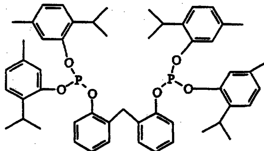
Ligand "E"
