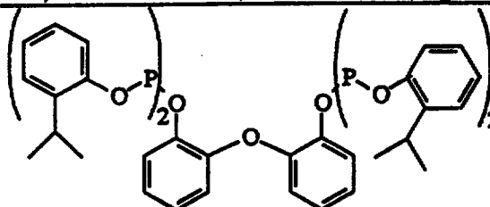
Ligand "K"
