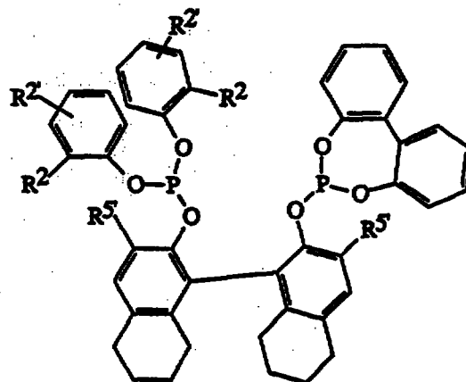
Formula VI
