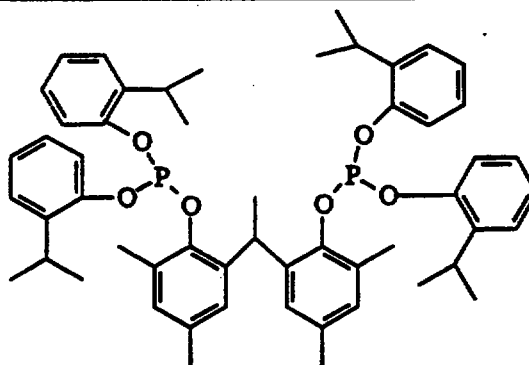
Ligand "D"
