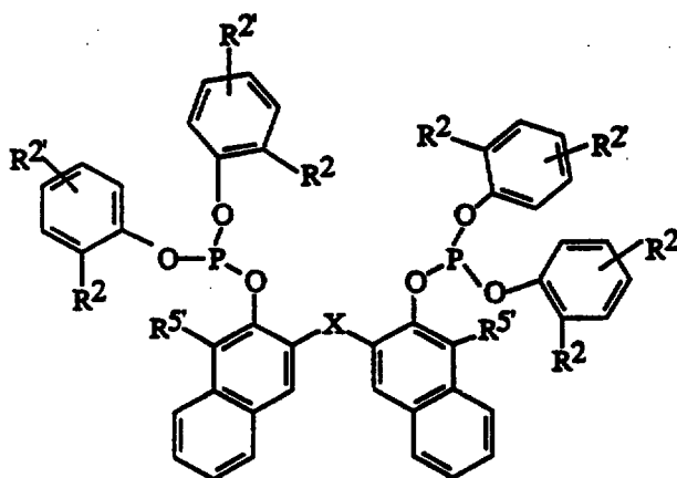
Formula III
