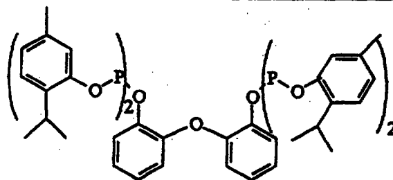
Ligand "L"
