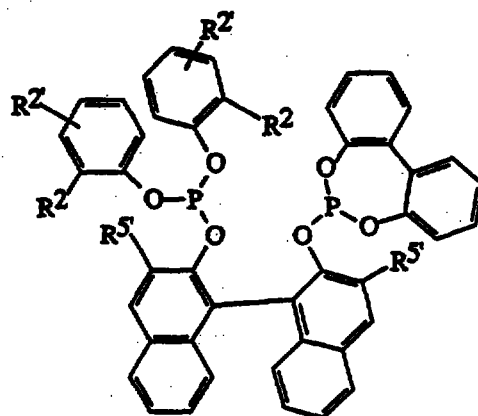
Formula IV
