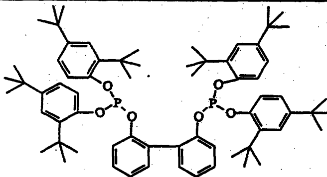
Ligand "A2"
