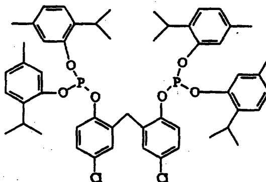
Ligand "G"
