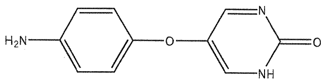
Compound 115
