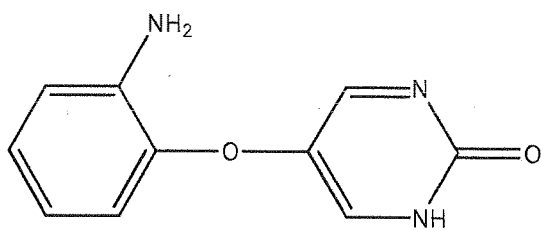
Compound 113
