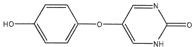
Compound 109
