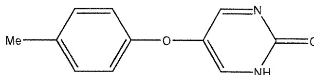
Compound 103
