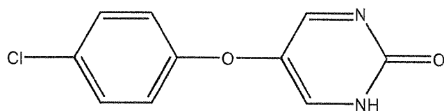
Compound 106
