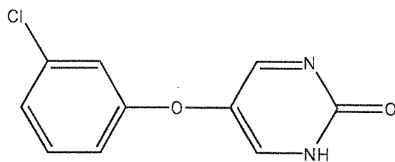
Compound 105
