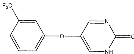
Compound 111
