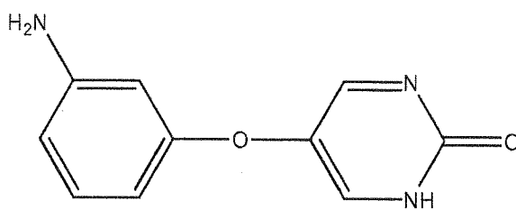
Compound 114
