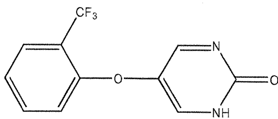
Compound 110
