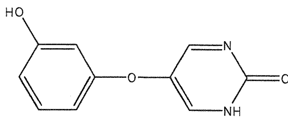
Compound 108
