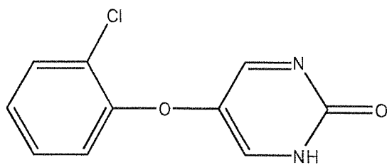
Compound 104
