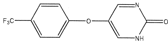
Compound 112
