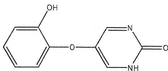
Compound 107
