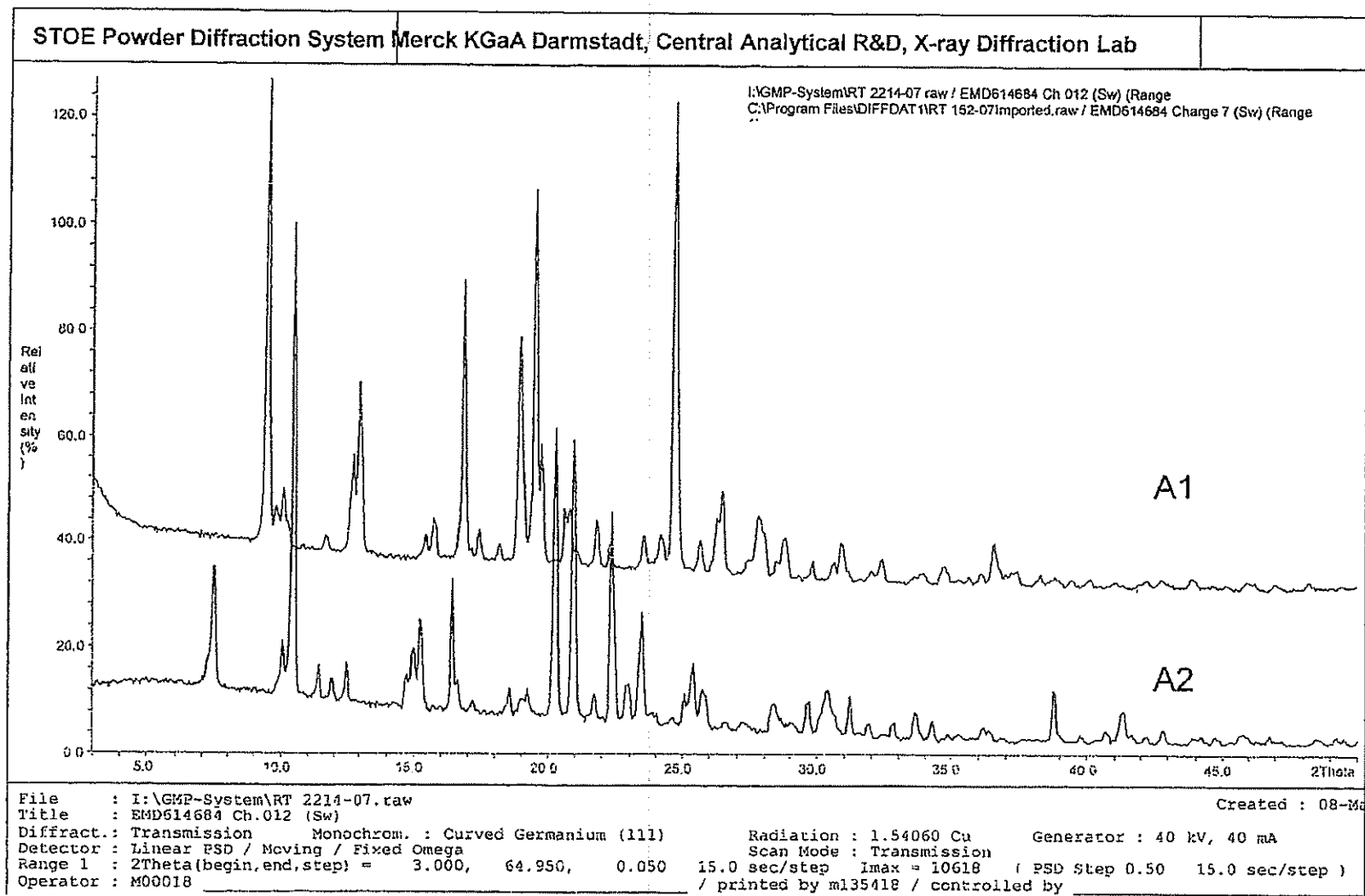
Fig.1 P-XRD of forms A1 and A2 of "C1"
