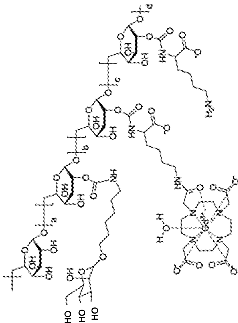
Target 7:Gd (counter ions not shown)
