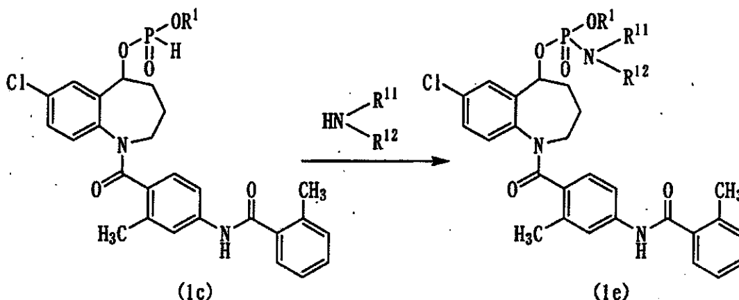
Reaction scheme-5
