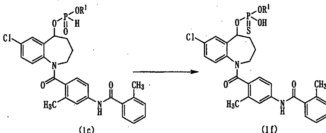
Reaction scheme-6
