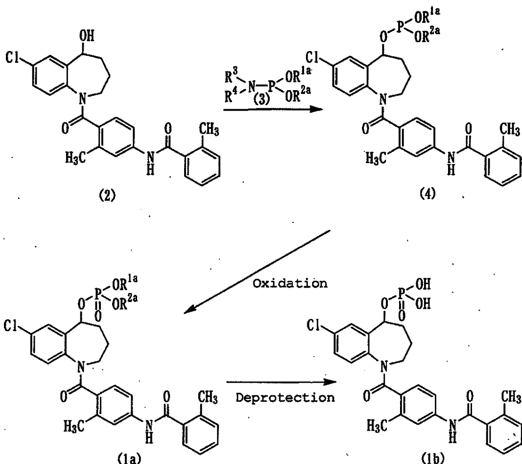
Reaction scheme-1
