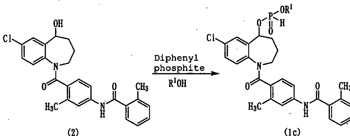
Reaction scheme-3
