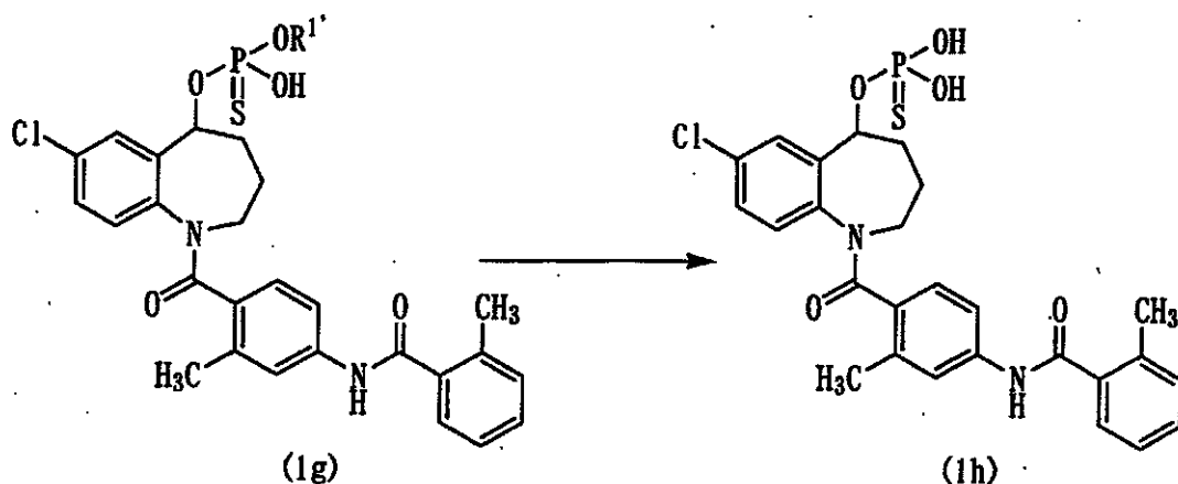
Reaction scheme-7
