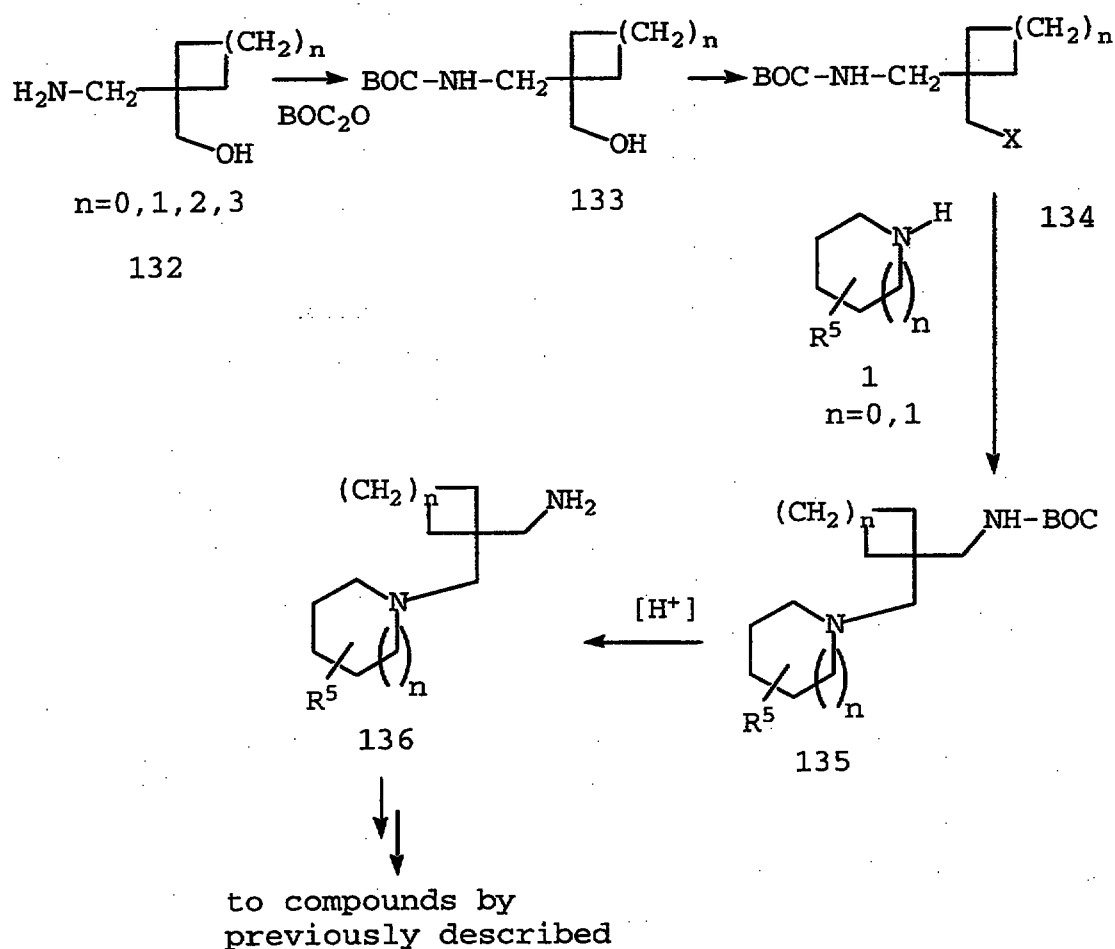
SCHEME 17
