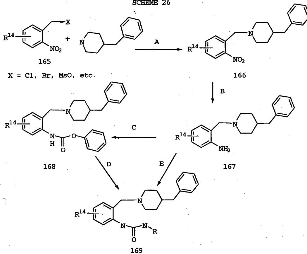
SCHEME 26
