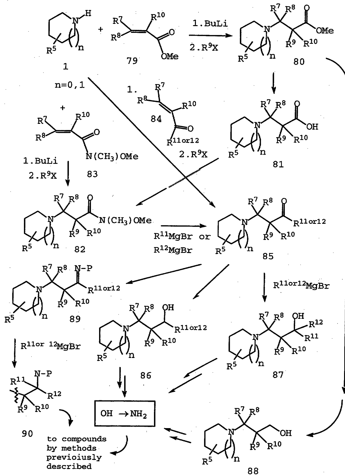
SCHEME 10
