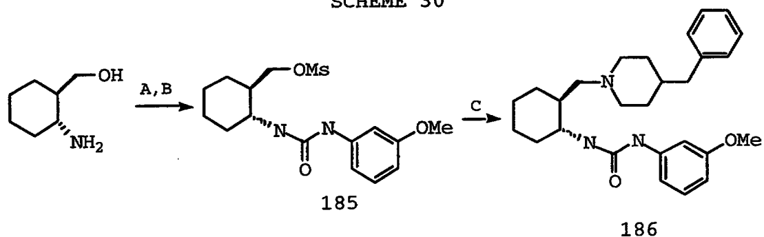
SCHEME 30
