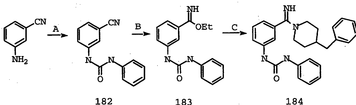
SCHEME 29
