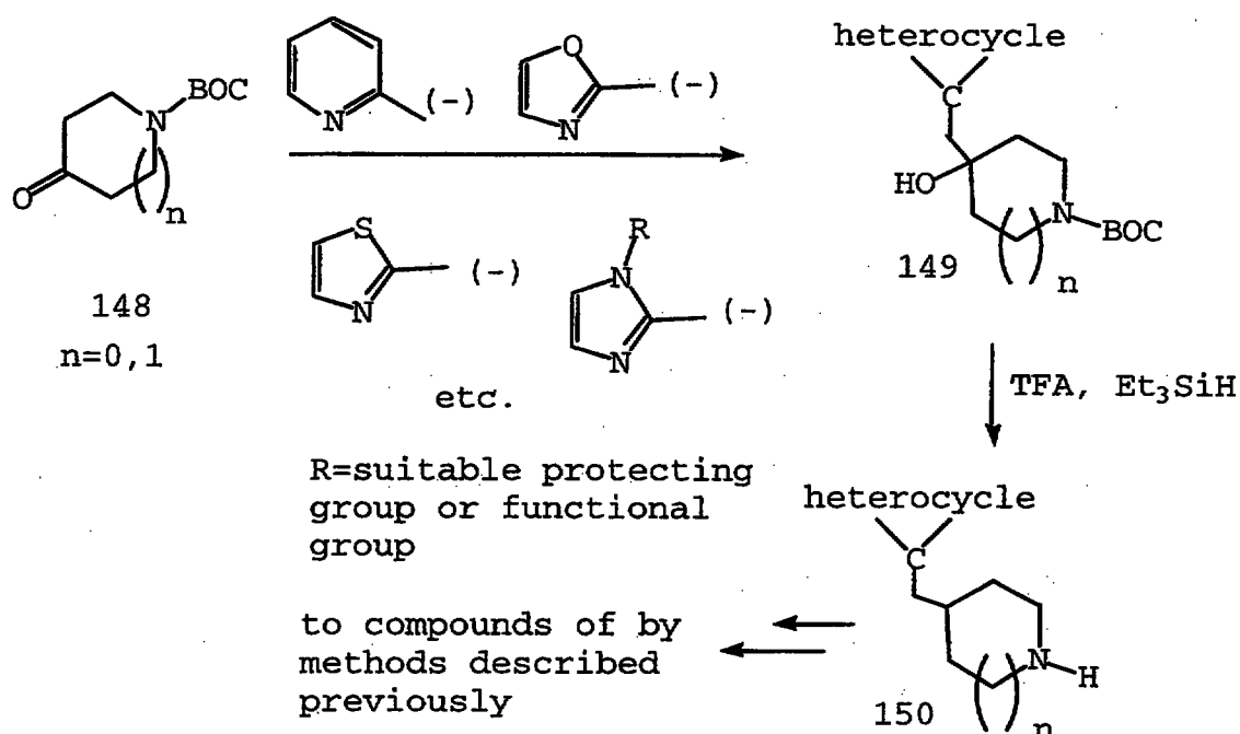
SCHEME 22
