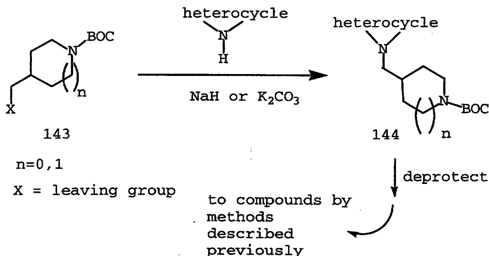
SCHEME 19
