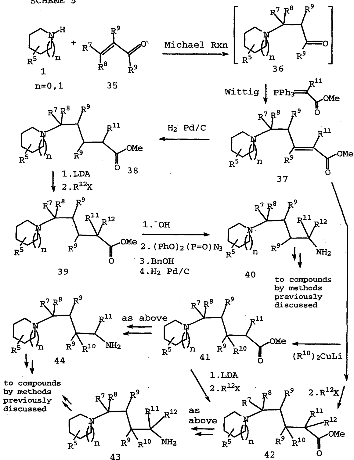
SCHEME 5
