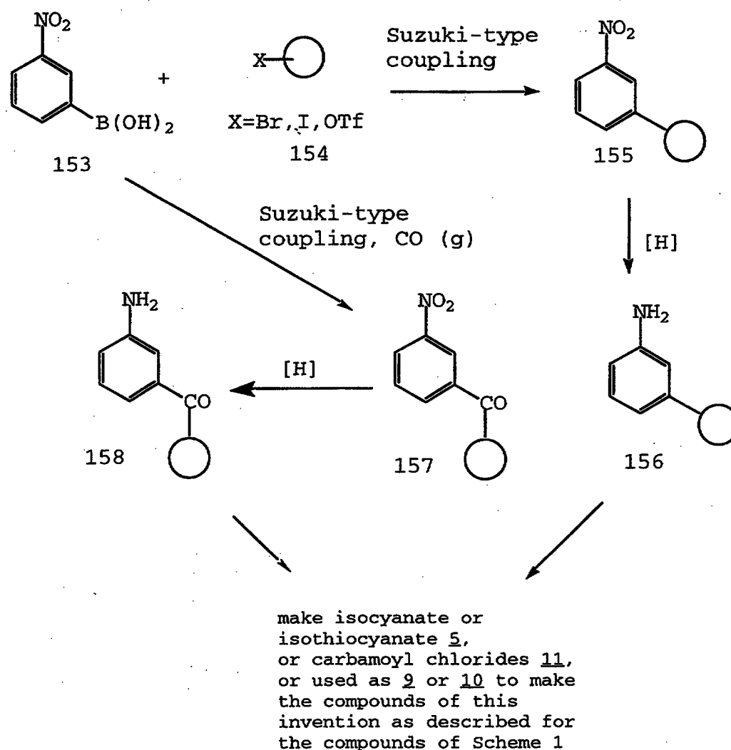
SCHEME 24
