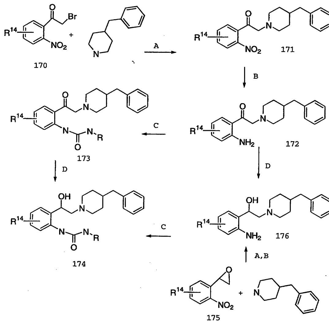
SCHEME 27
