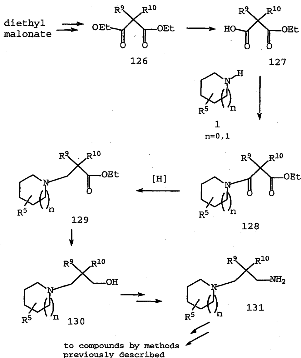
SCHEME 16
