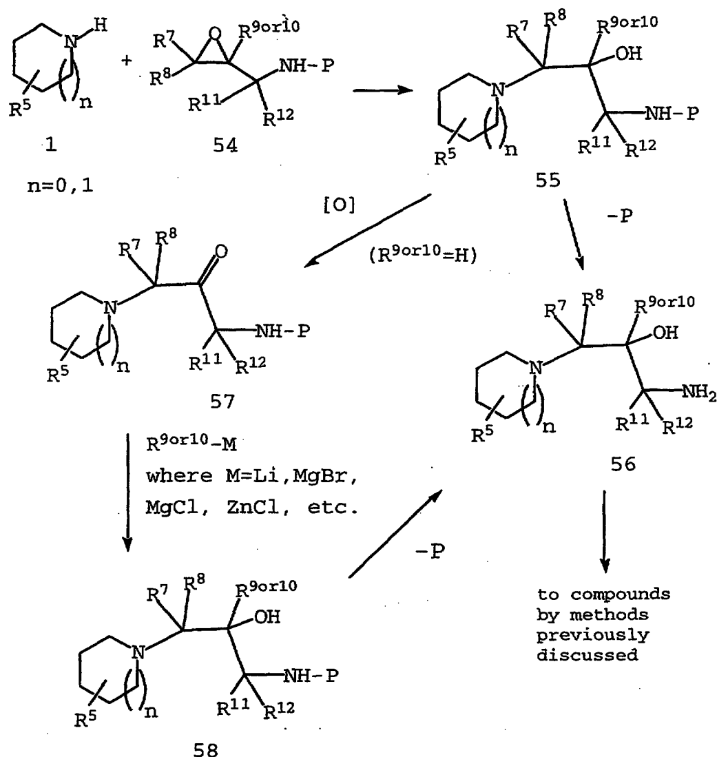
SCHEME 8
