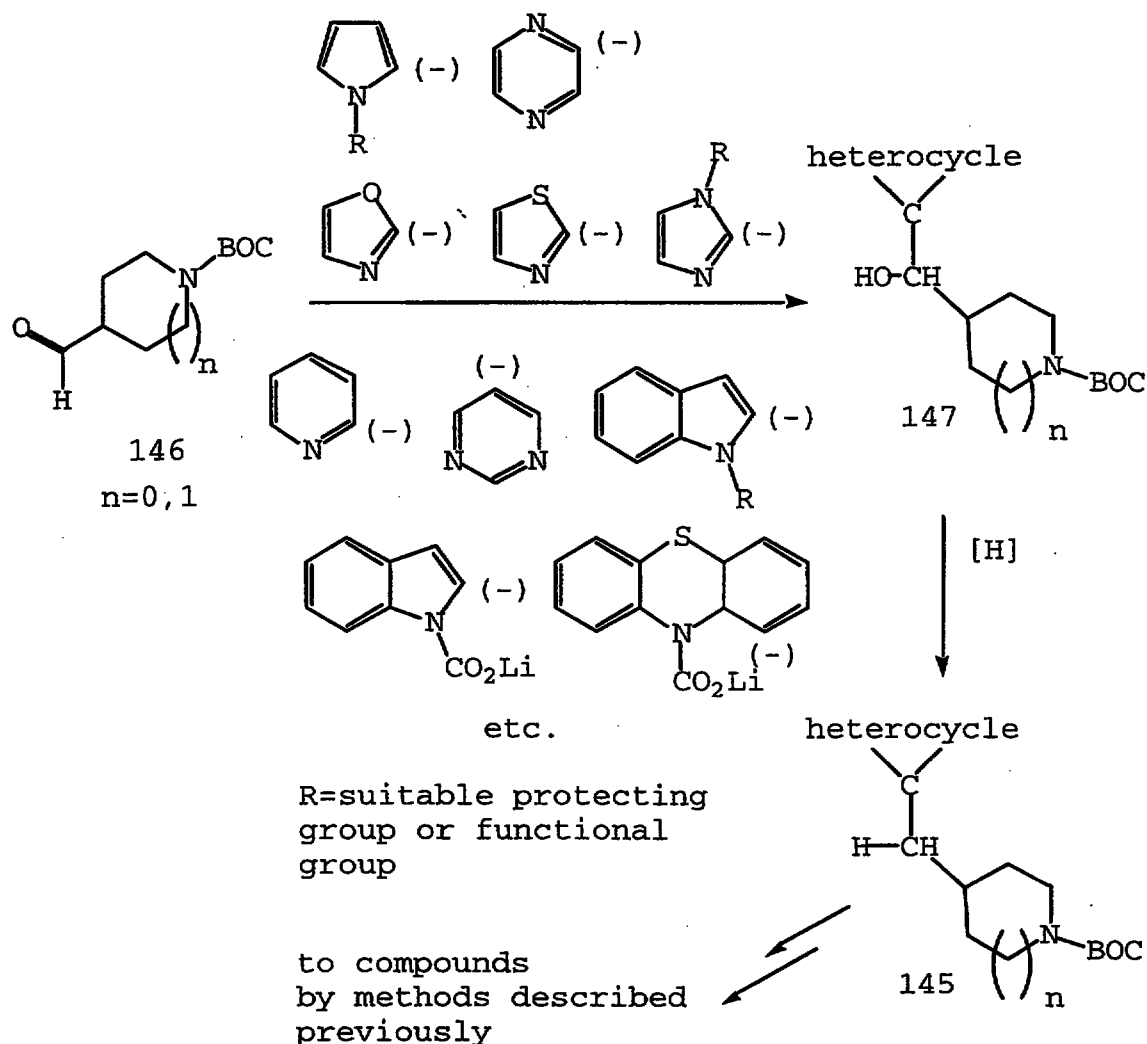
SCHEME 21
