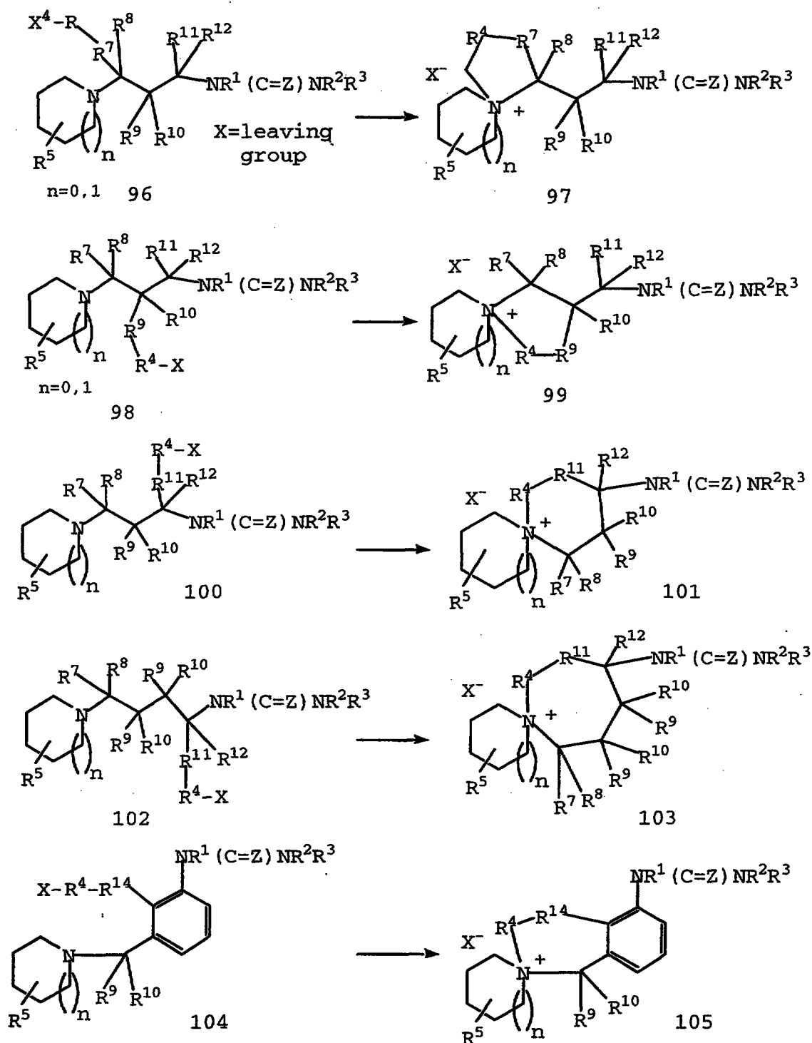
SCHEME 12
