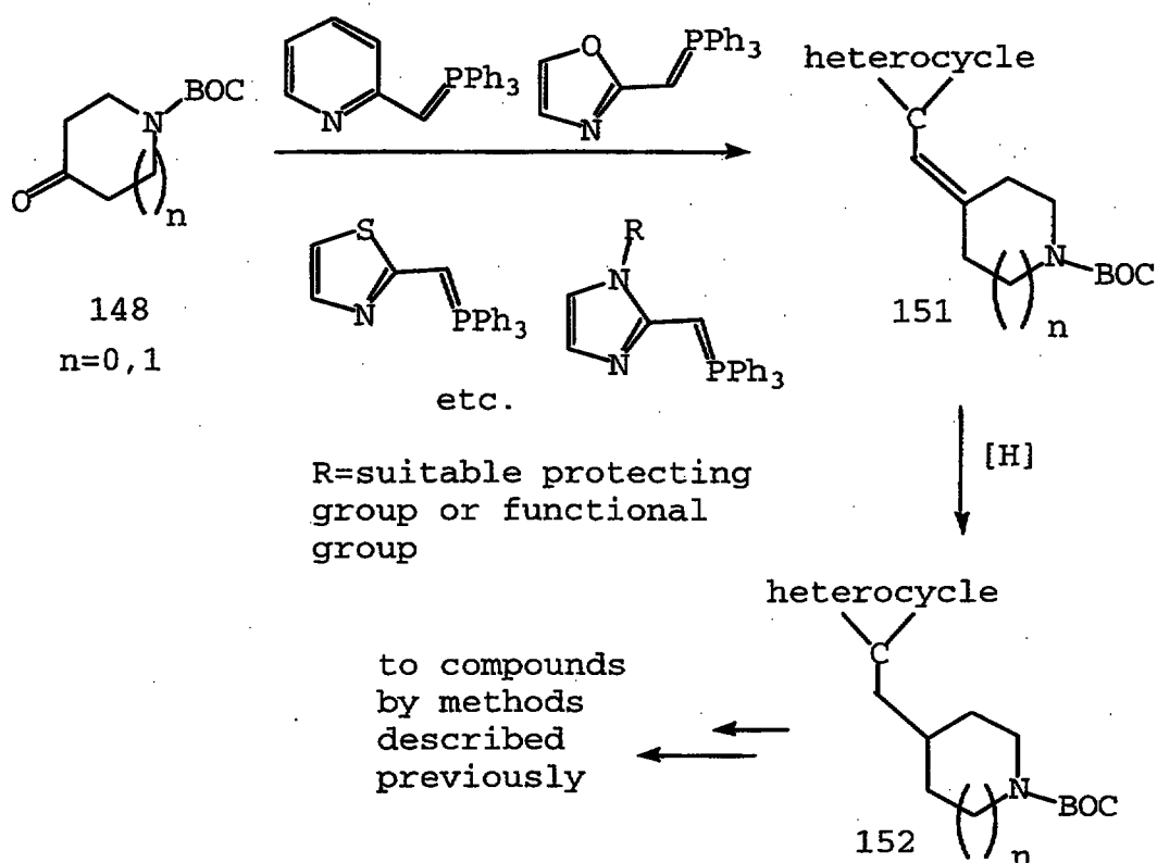
Scheme 23
