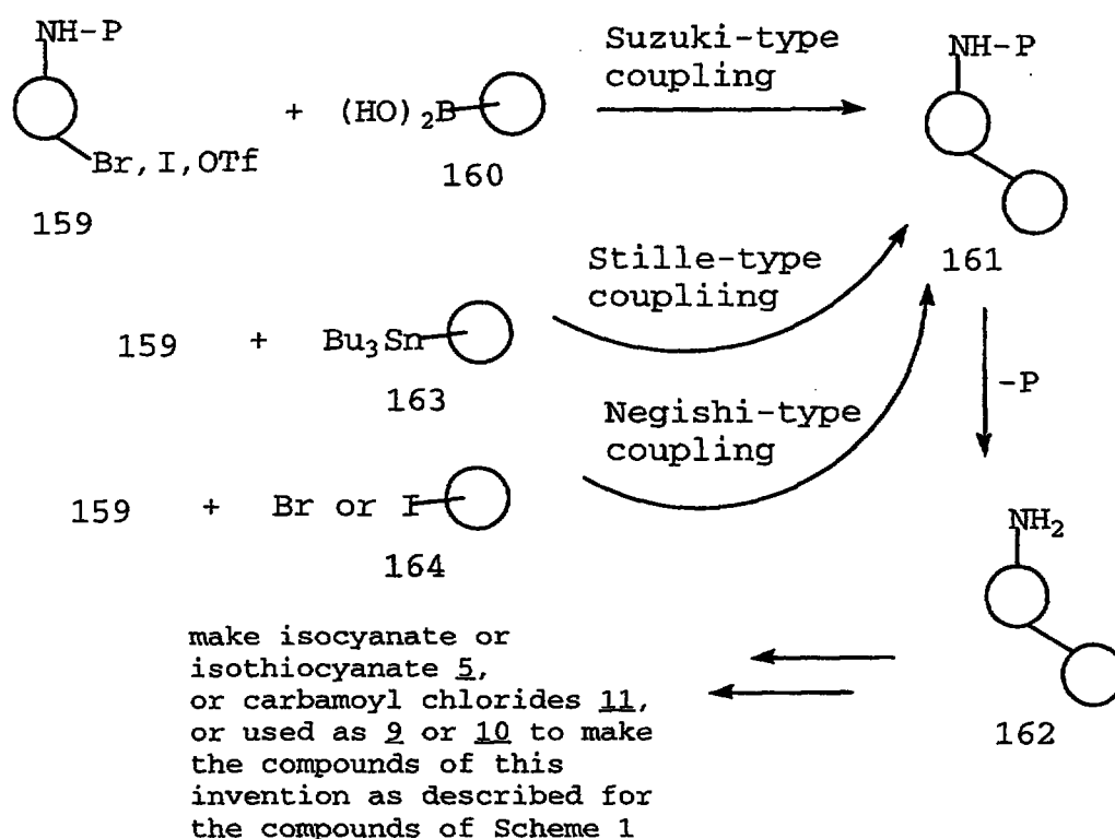
SCHEME 25
