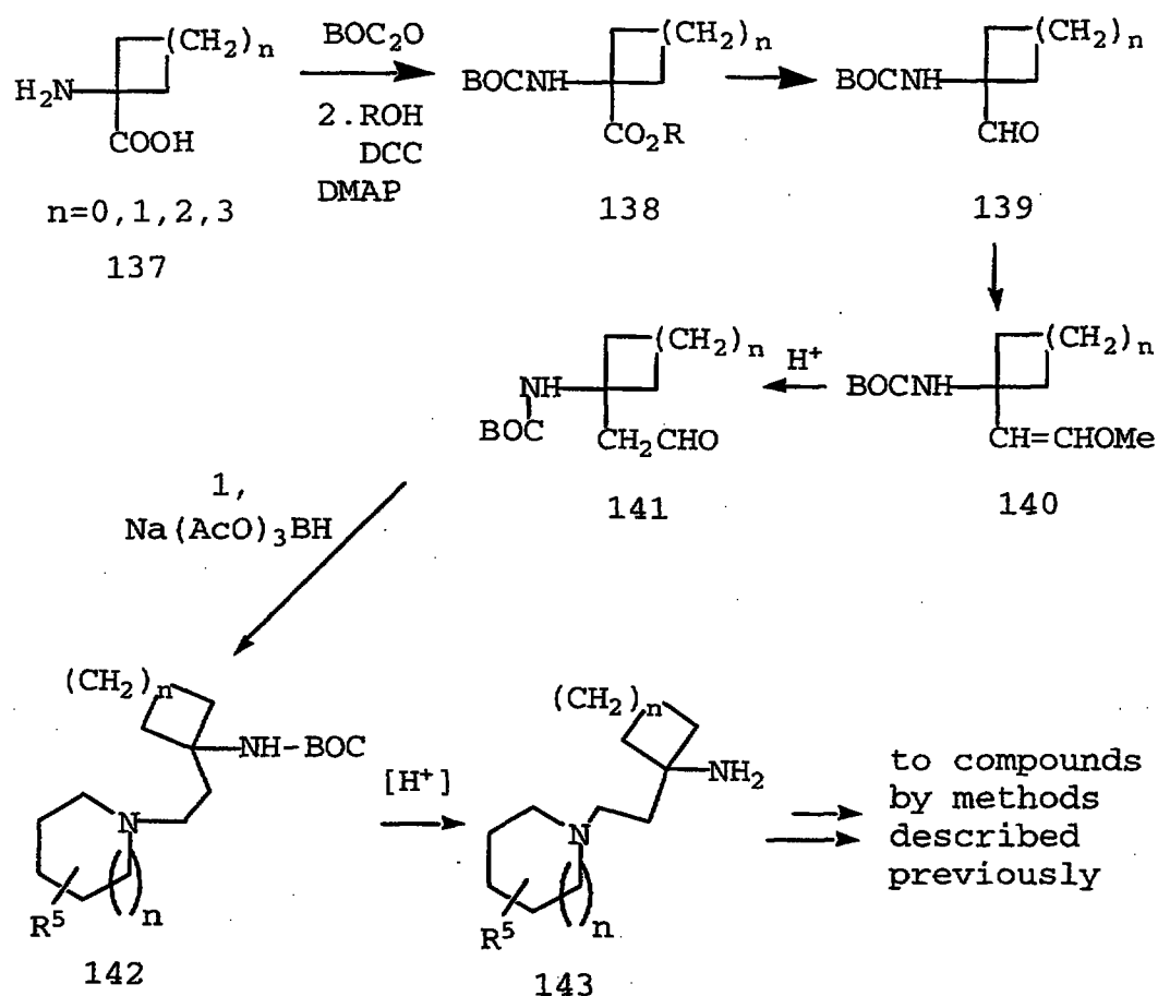
SCHEME 18
