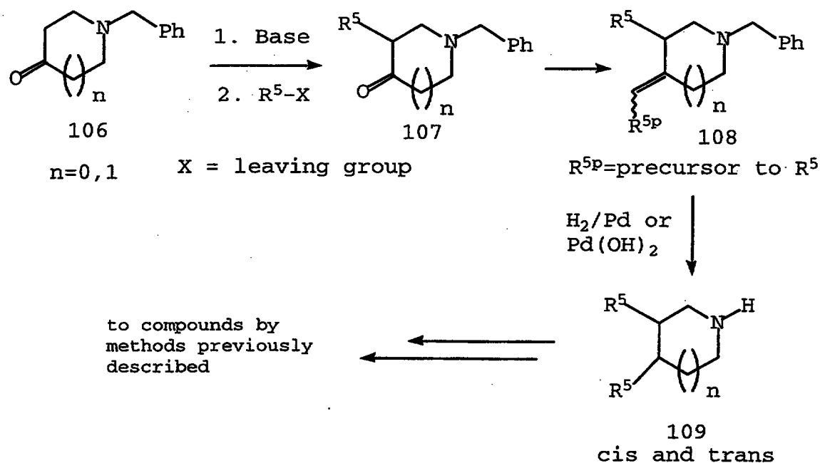
SCHEME 13
