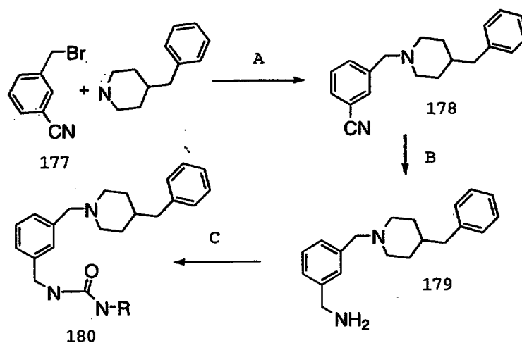
SCHEME 28
