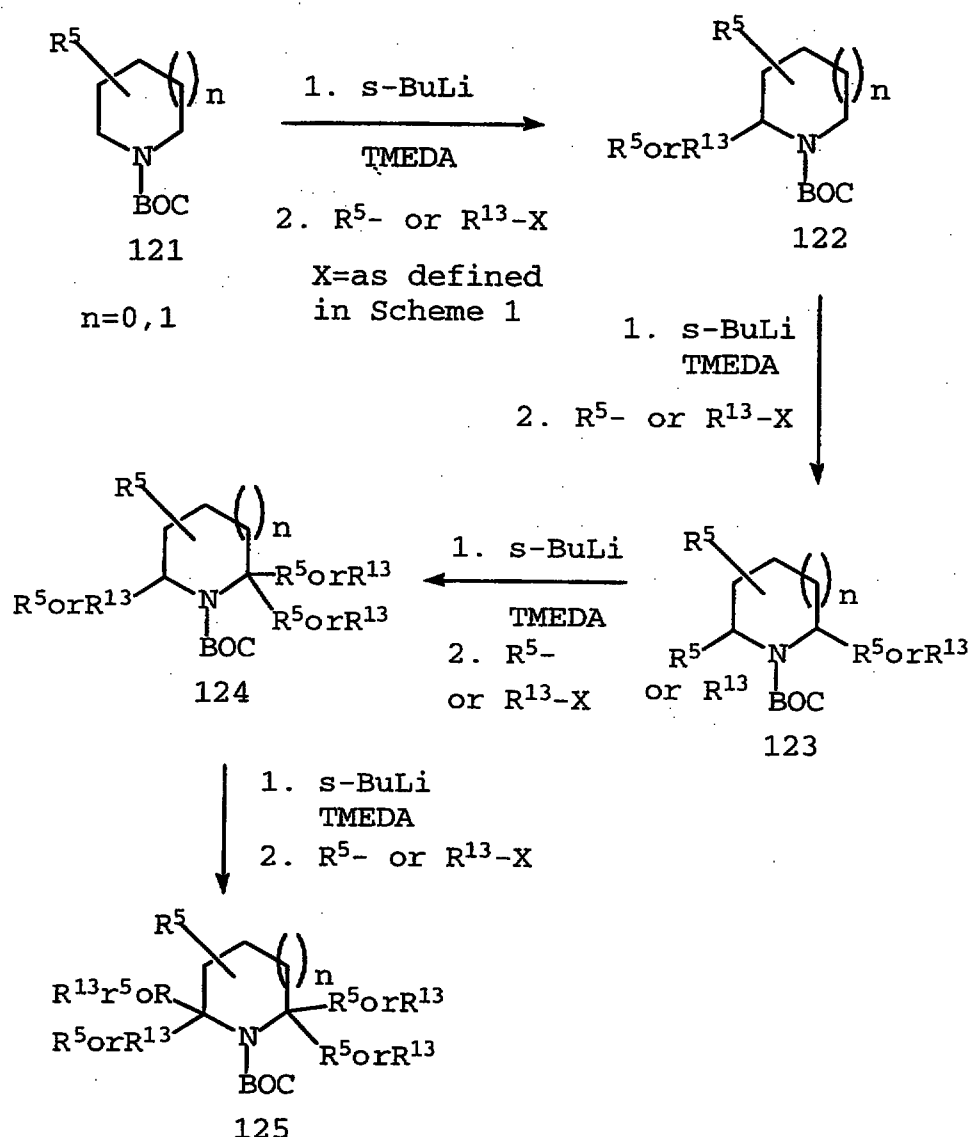
SCHEME 15
