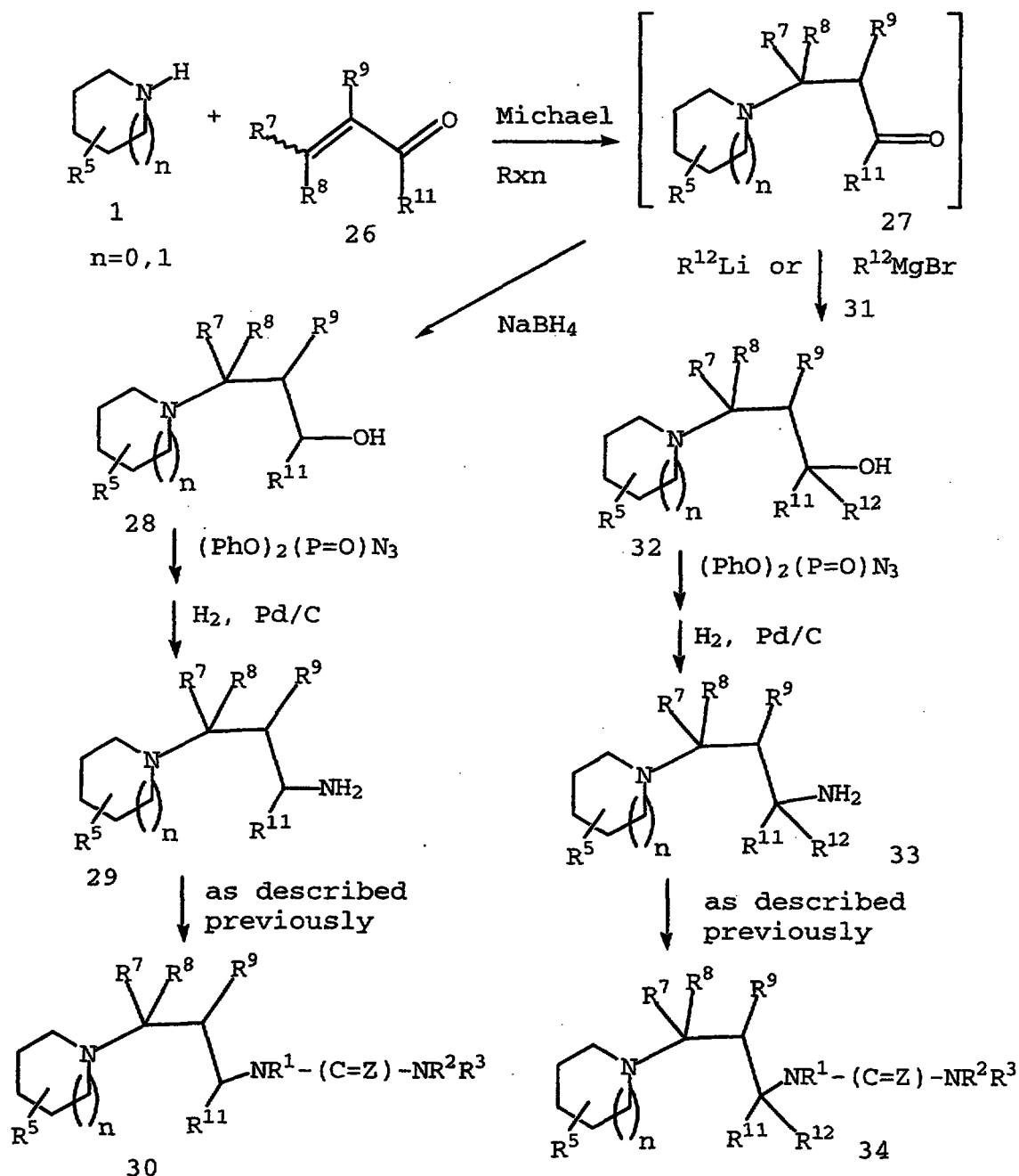
SCHEME 4
