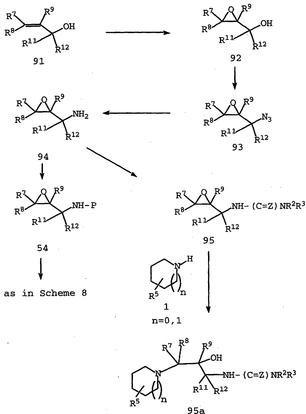
SCHEME 11
