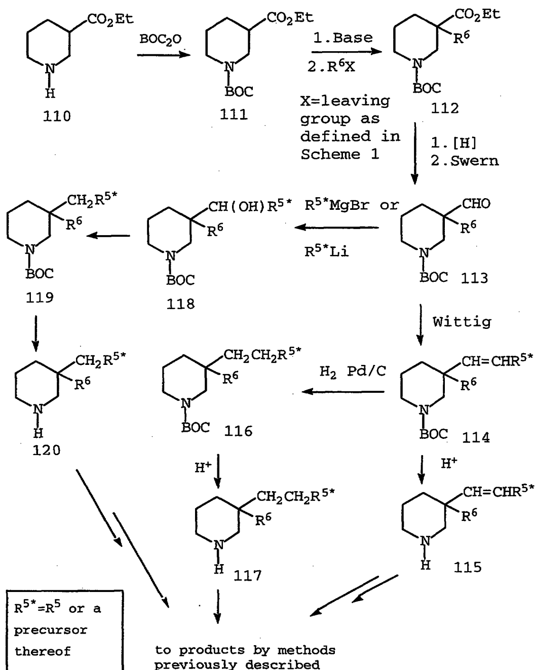
SCHEME 14
