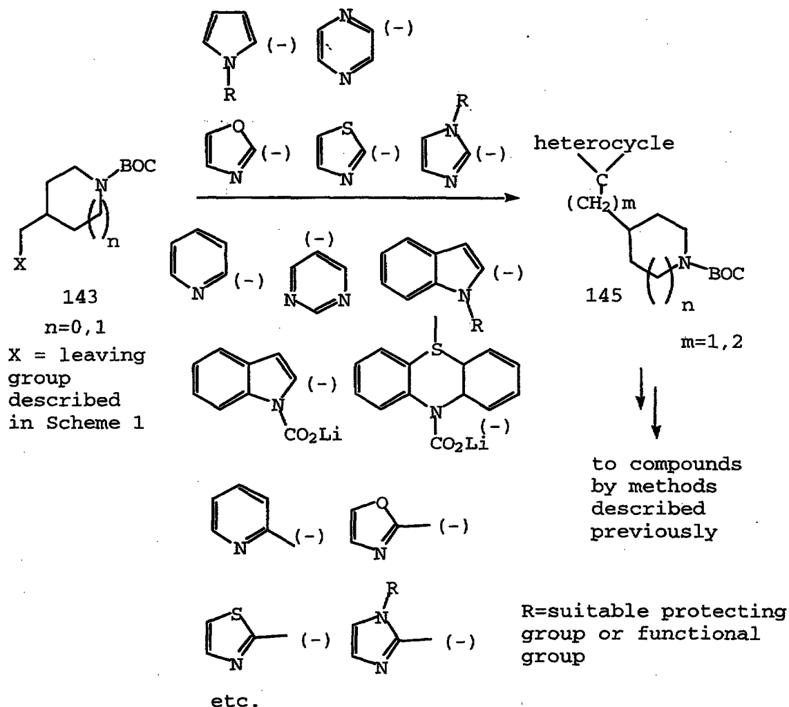
SCHEME 20
