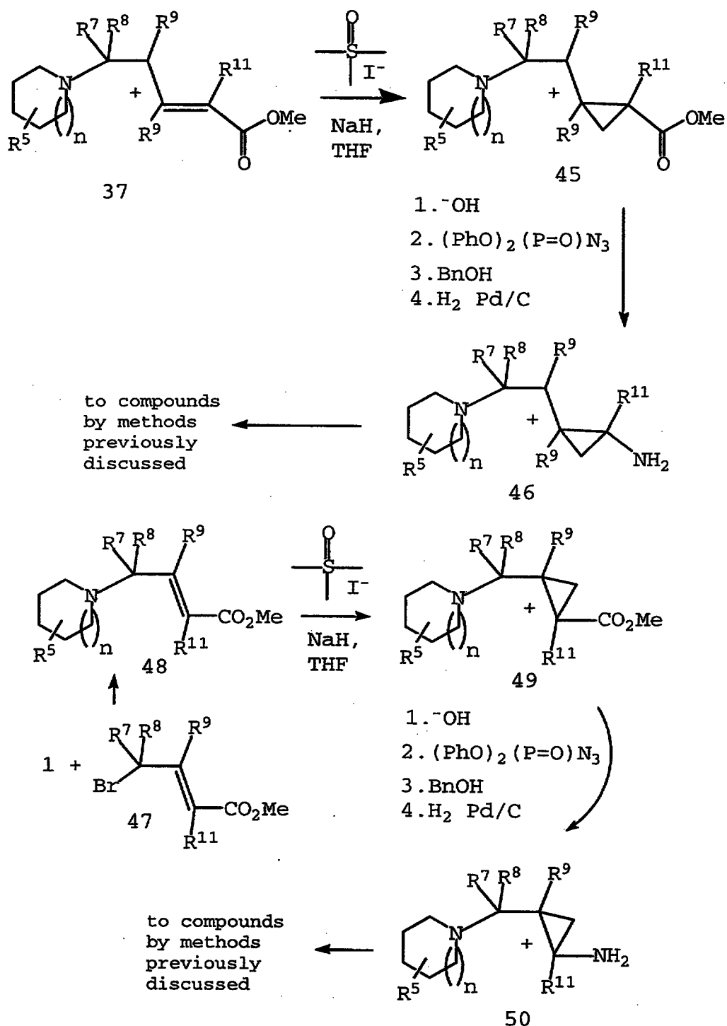
SCHEME 6
