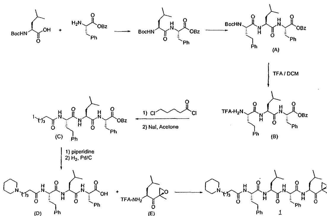
Scheme 1: Synthesis of Example 1
