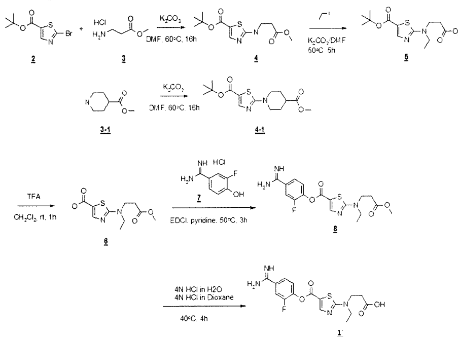
[Reaction Scheme 1]
