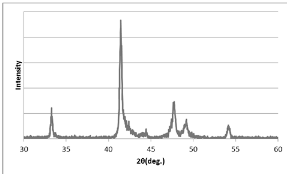
Example 5 XRD Profile
