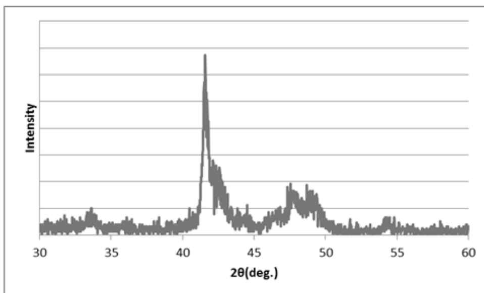
Example 1 XRD Profile
