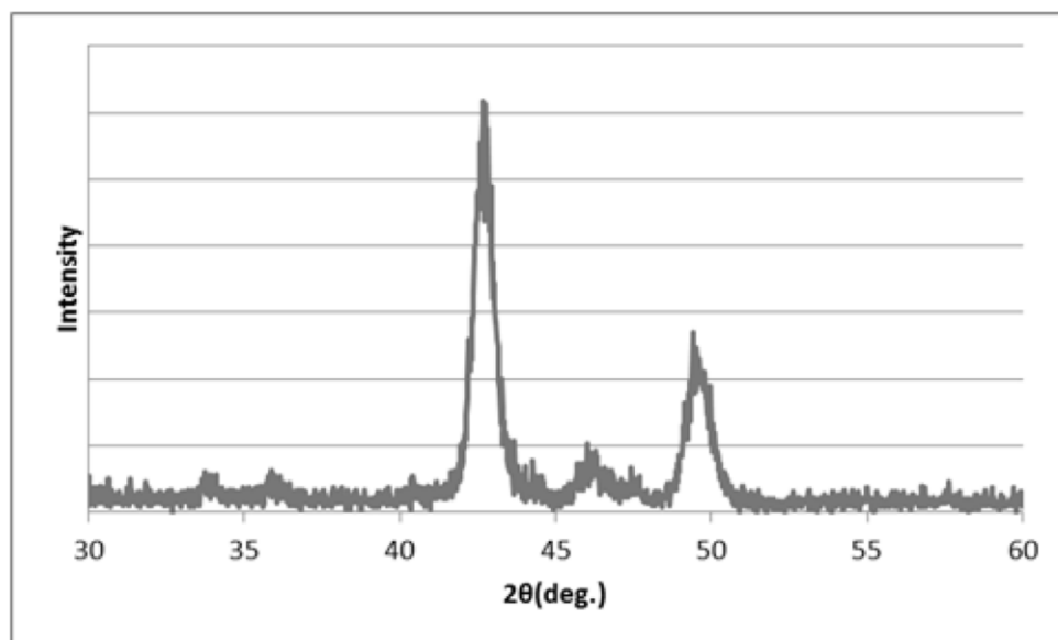
Comparative Example 1 XRD Profile
