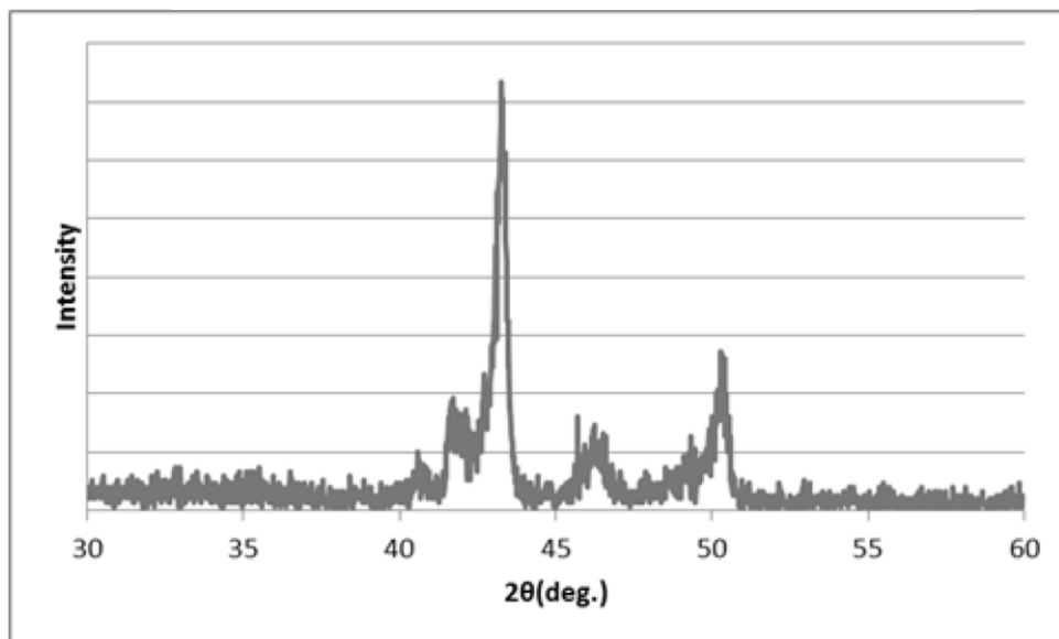
Comparative Example 3 XRD Profile
