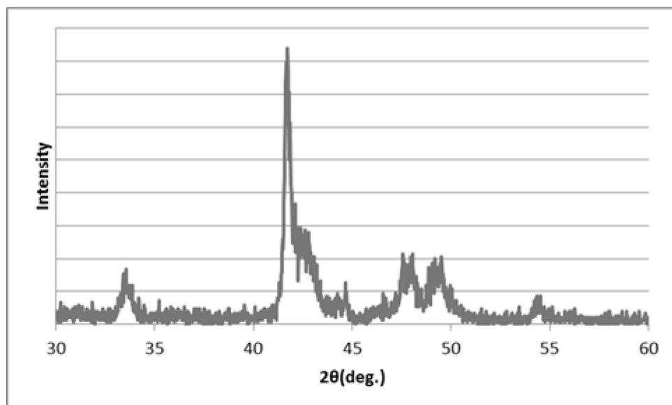
Example 2 XRD Profile
