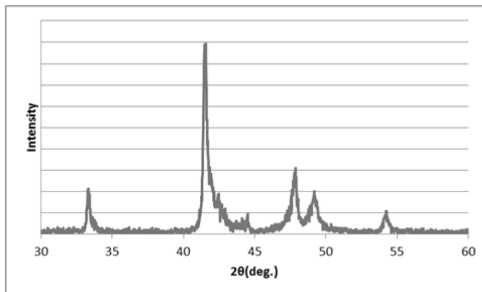
Example 7 XRD Profile
