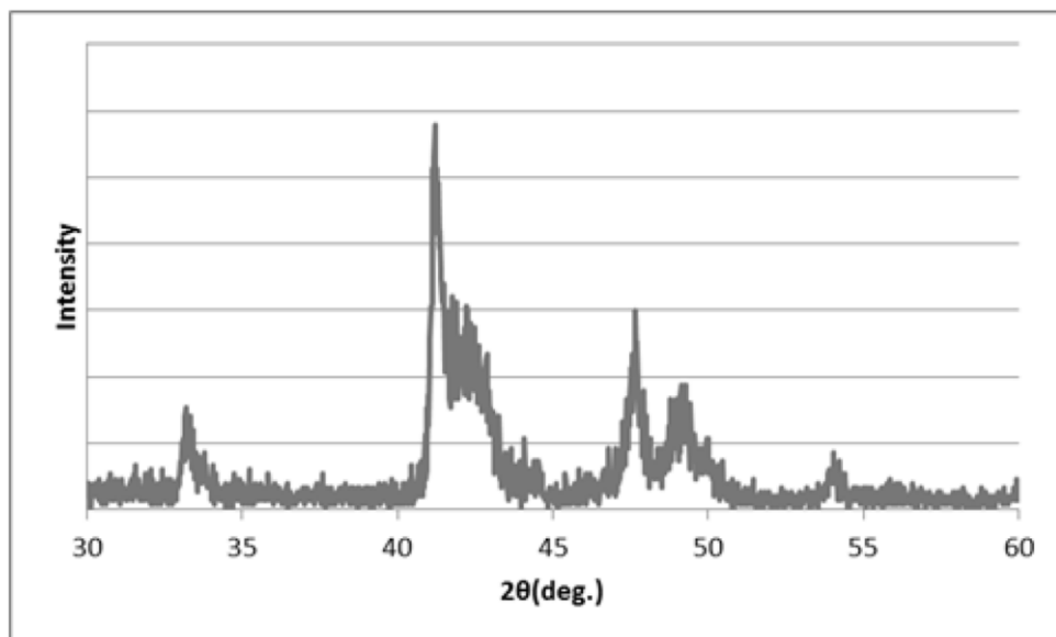
Example 3 XRD Profile
