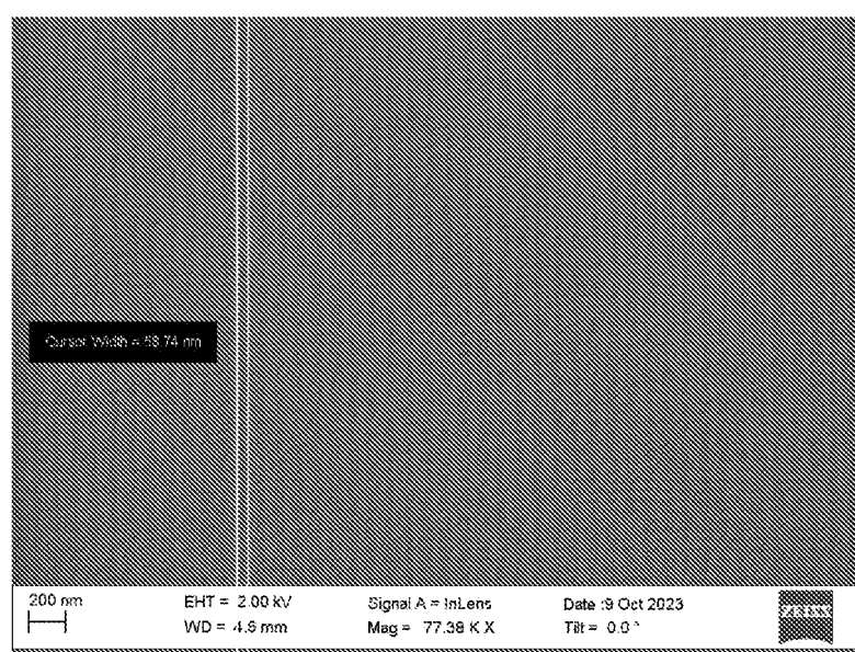
Fig.5. EBEAM images
