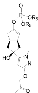
Compound XI
