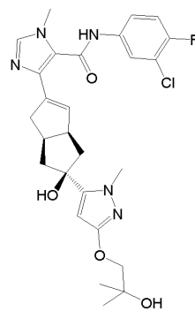
Compound 3.4a
