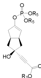
Compound IX
