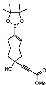
Compound 3.1
