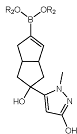
Compound V ,
