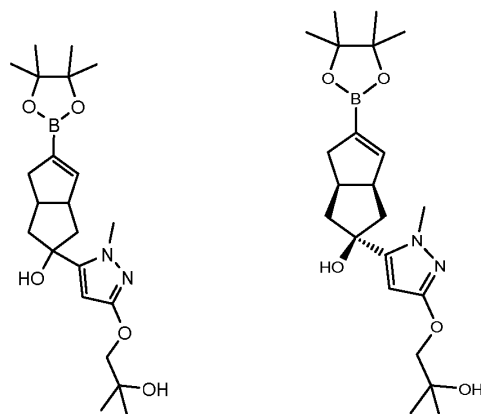
Compound 3.3
