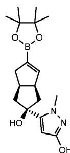
Compound 3.2a
