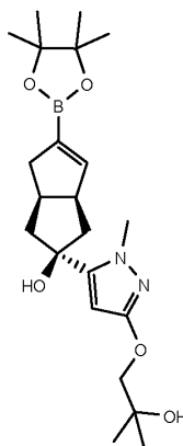
Compound 3.3a
