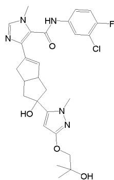
Compound 3.4
