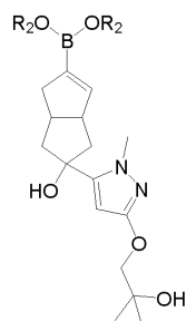
Compound VII
