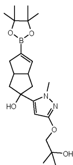
Compound 3.3
