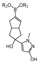
Compound V
