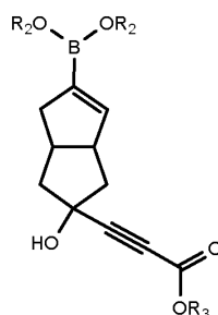
Compound IV
