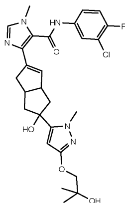
Compound 3.4
