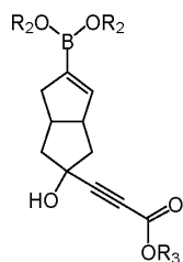
Compound IV
