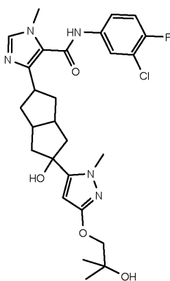
Compound I,
