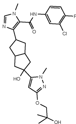
Compound I,
