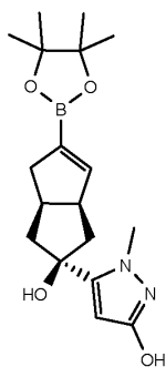
Compound 3.2a
