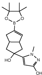
Compound 3.2
