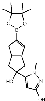
Compound 3.2
