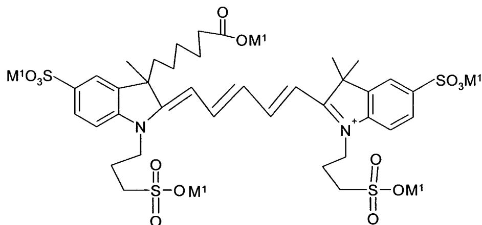
Alexa Fluor™ 647
