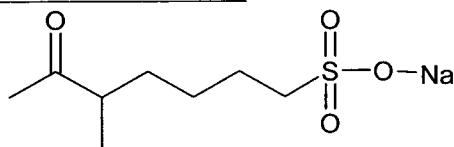
Cy5**
