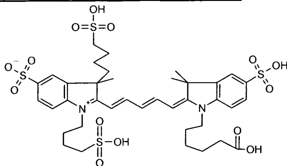
Cy5**
