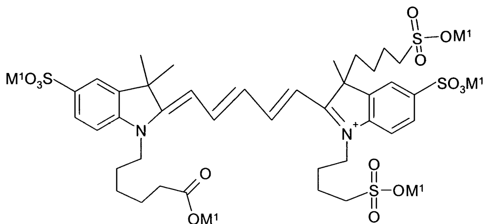
Cy5**
